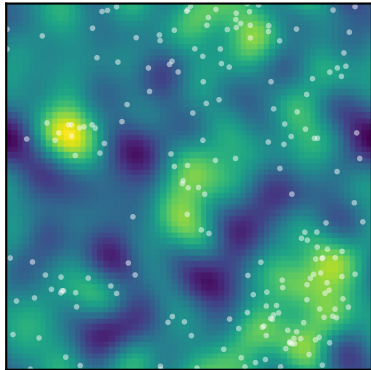
true log-intensity
