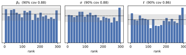
Figure 3: Simulation-based calibration rank histograms with 90% coverage in the titles (uniform ranks and the dashed line indicate calibration; grey band is the 99% envelope). Coverage is near nominal for all three parameters; the range \ell is the most over-confident, a stated limitation.
