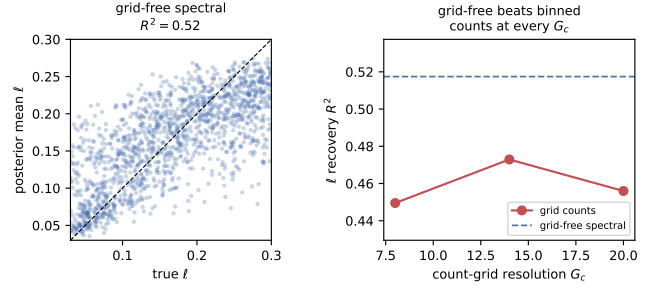
Figure 1: Correlation-range recovery. Left: true versus posterior-mean \ell with grid-free spectral conditioning ( R^2 = 0.52 ). Right: \ell recovery of the binned-count baseline as a function of grid resolution G_c ; it stays flat and consistently below the grid-free reference (dashed) at every resolution, so refining the grid does not recover the lost range information. Only the conditioning summary differs – simulator, spectral target, whitening, and flow sampler are identical.
