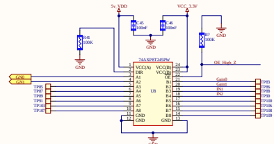
Level Converter including 3-state output OE="1" - output =High Z
