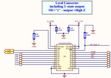
Level Converter
