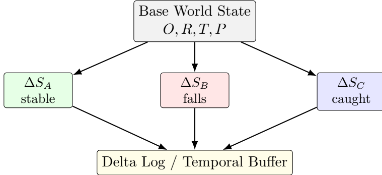
Figure 7: Supplementary branch-memory schematic. A WPU shares the base state and stores branch-specific deltas, reducing memory from O(BN) to O(N + B\Delta) when branches are local.
