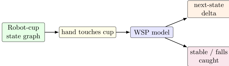
Figure 4: Validation task. The model observes an object-relation state graph and an event, then predicts next-state deltas and future branch probabilities.
