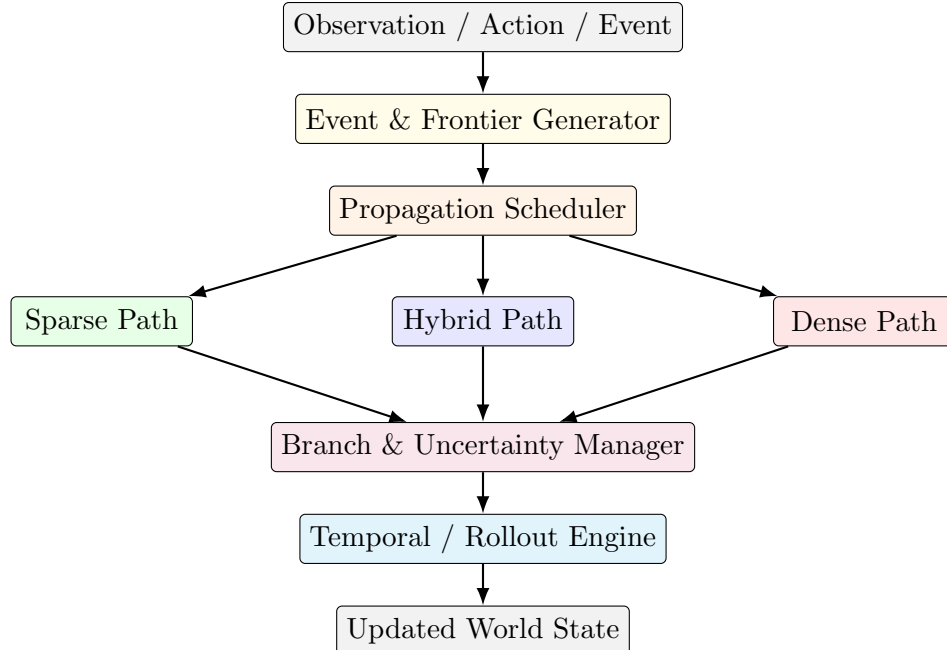
Figure 2: WPU schematic. Events generate frontiers, the scheduler chooses a sparse, hybrid, or dense execution path, and branches are maintained as deltas over shared state.
