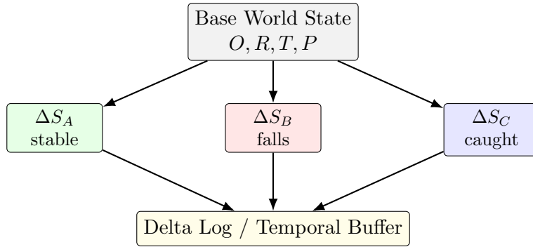
Figure 7: Supplementary branch-memory schematic. A WPU shares the base state and stores branch-specific deltas, reducing memory from O(BN) to O(N + B\Delta) when branches are local.
