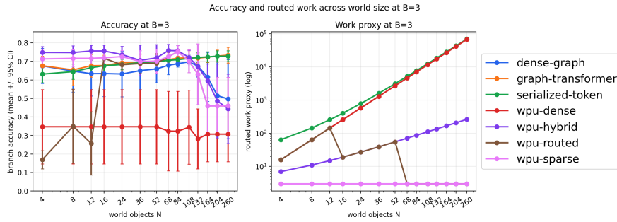
(b) Accuracy and routed work versus world size at B = 3 , aggregated over seeds.
