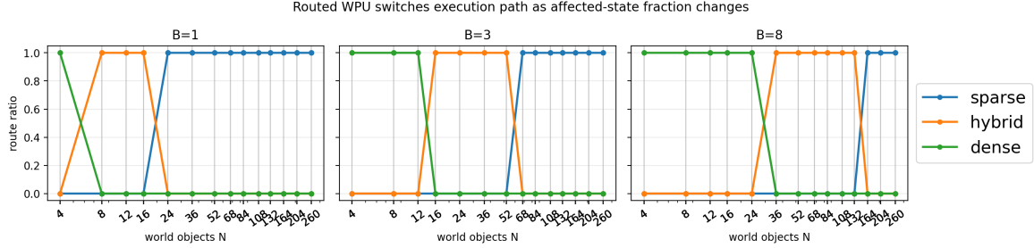
(a) Routed WPU execution-path ratios as world size and branch pressure vary.
