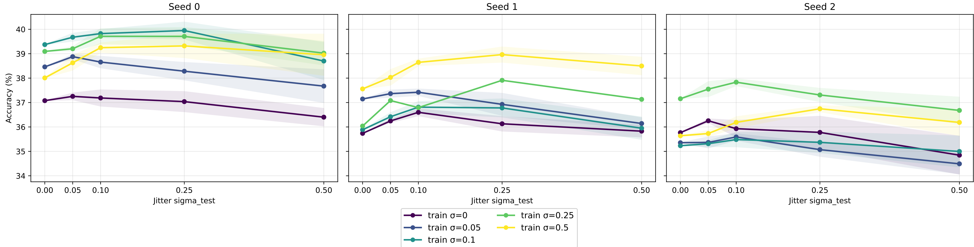
SSC sparse (sparsity=0.96): Jitter robustness by seed and train sigma
