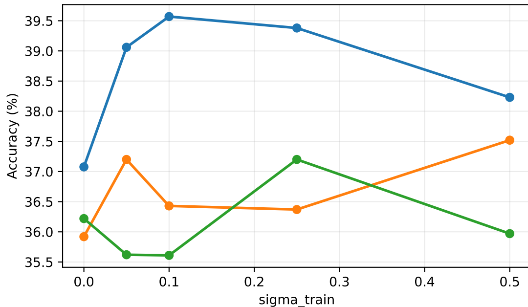
Best test accuracy from training
