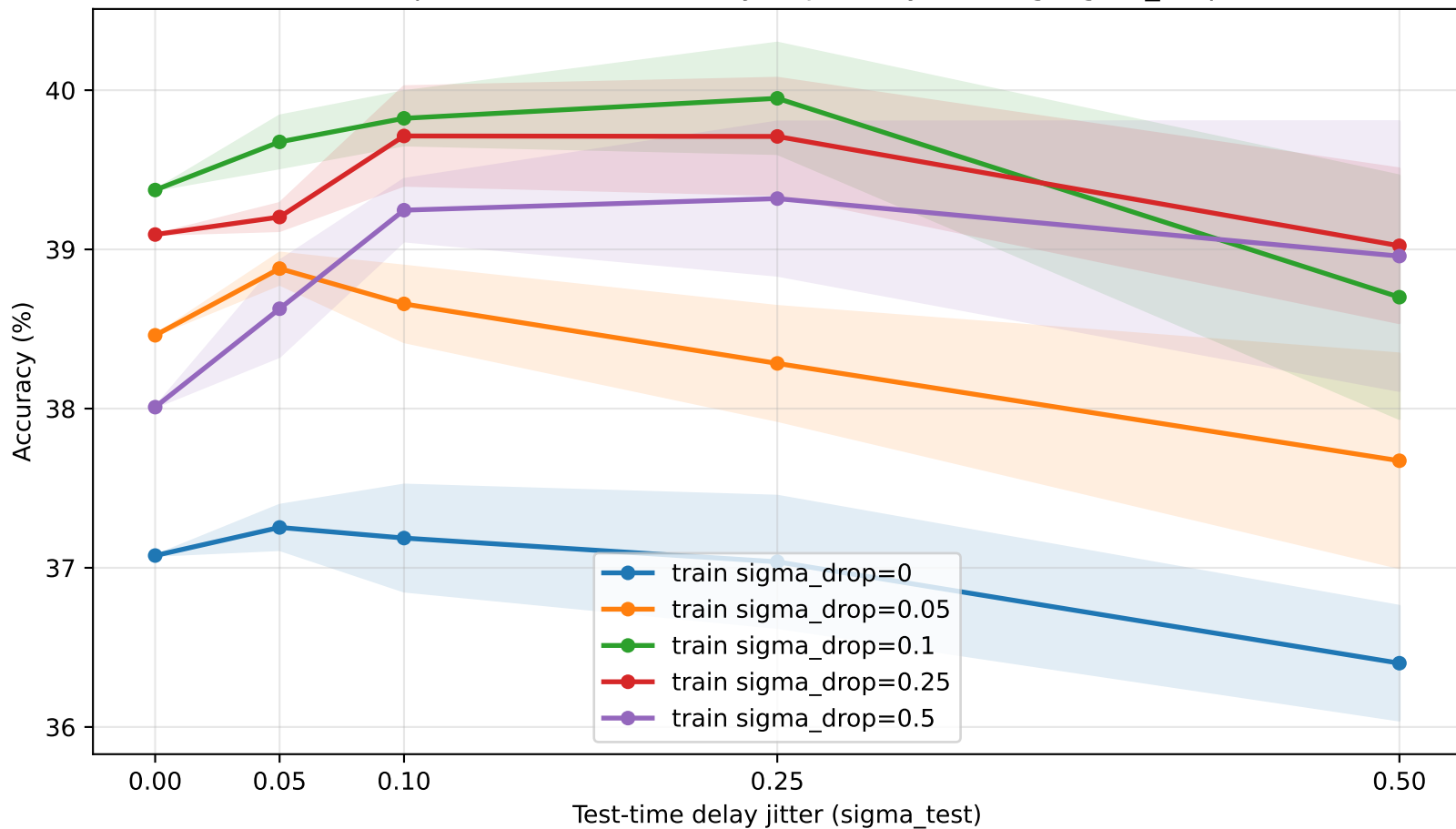
SSC Sparse Seed-0: Accuracy vs Jitter by Training sigma_drop
