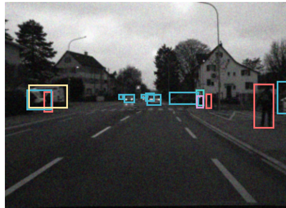
Severity 1
