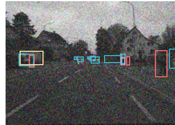
Severity 5
