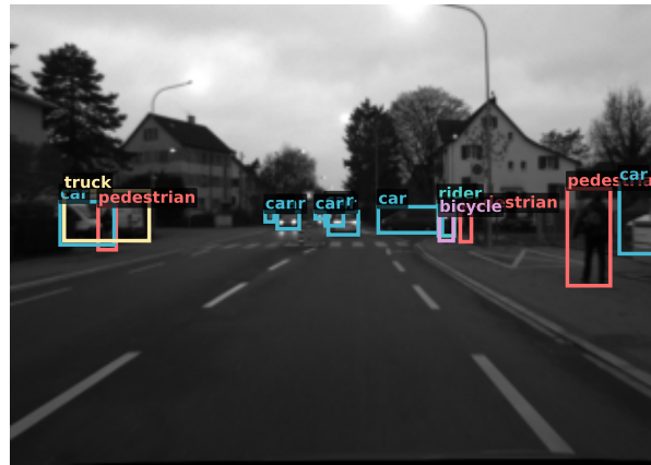
Clean
