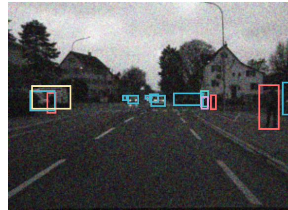
Severity 3
