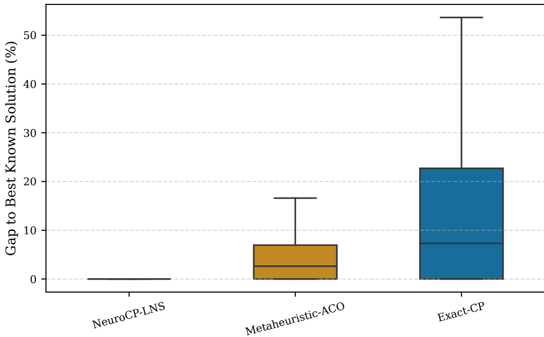
Optimality Gap Distribution
