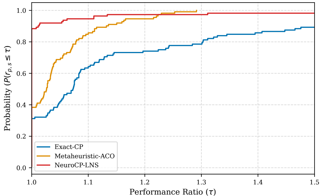
Performance Profile (Cost)
