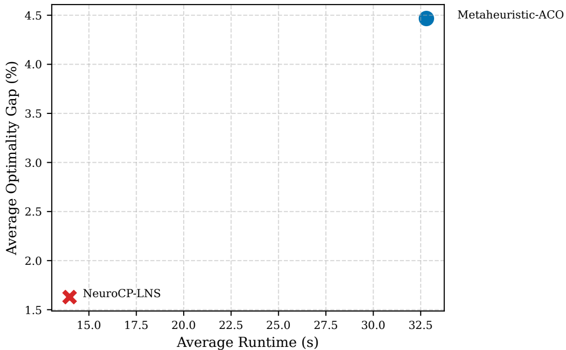
Efficiency Frontier
