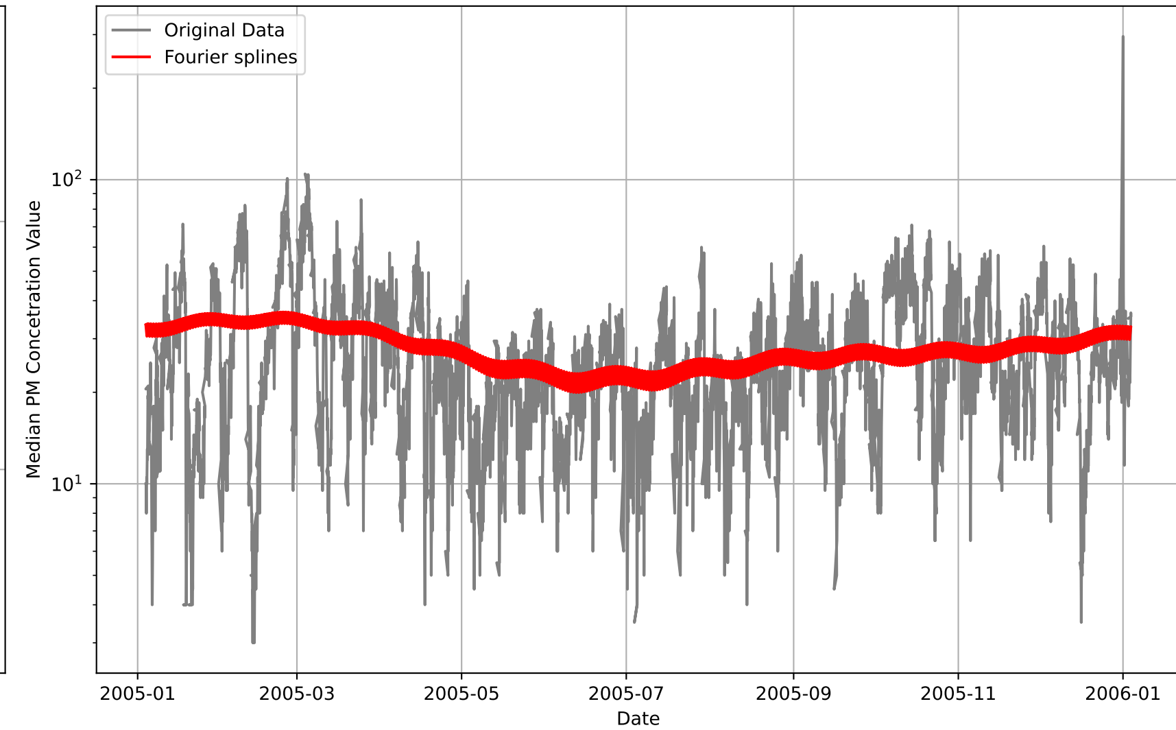
Data vs Fourier splines (1Year)
