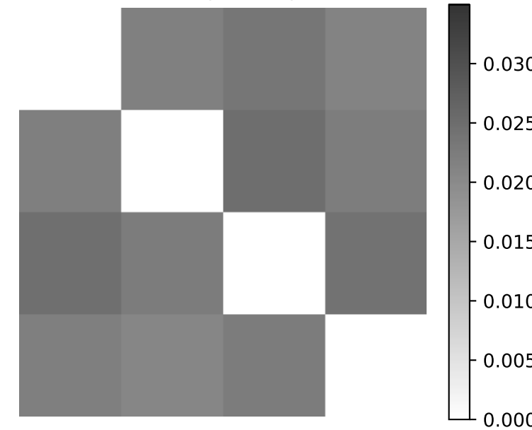
MAE (T=100)
