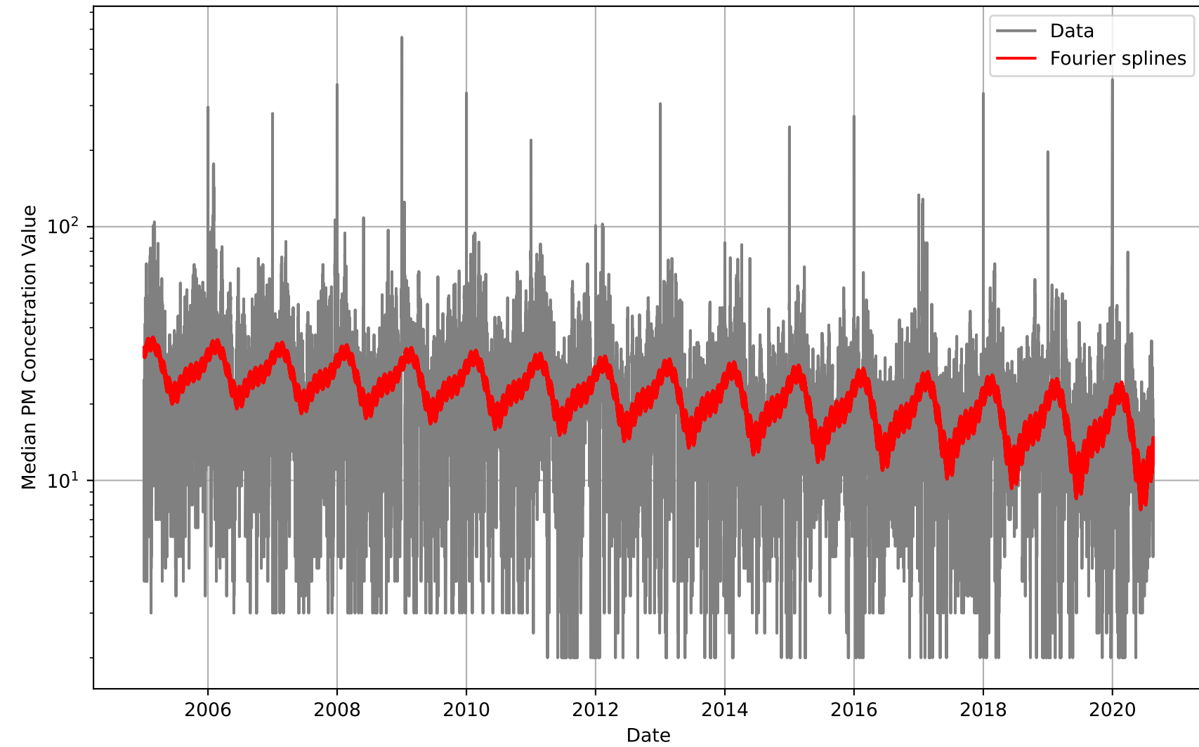
Data vs Fourier splines
