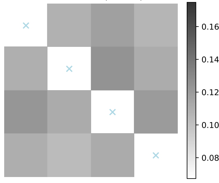
Relative MAE (T=100)
