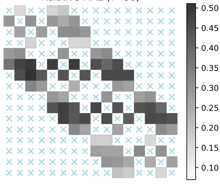
Relative MAE (T=50)
