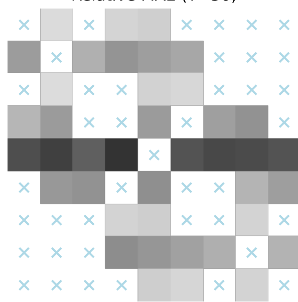
Relative MAE (T=50)
