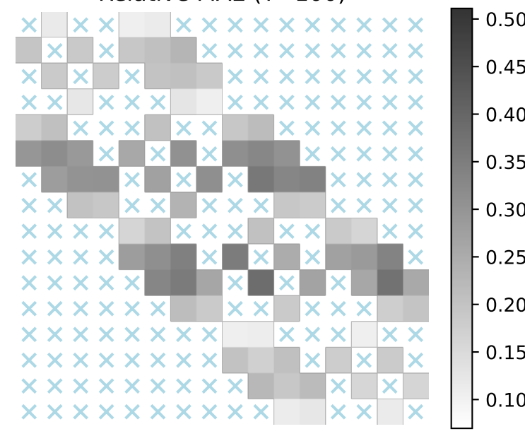
Relative MAE (T=100)
