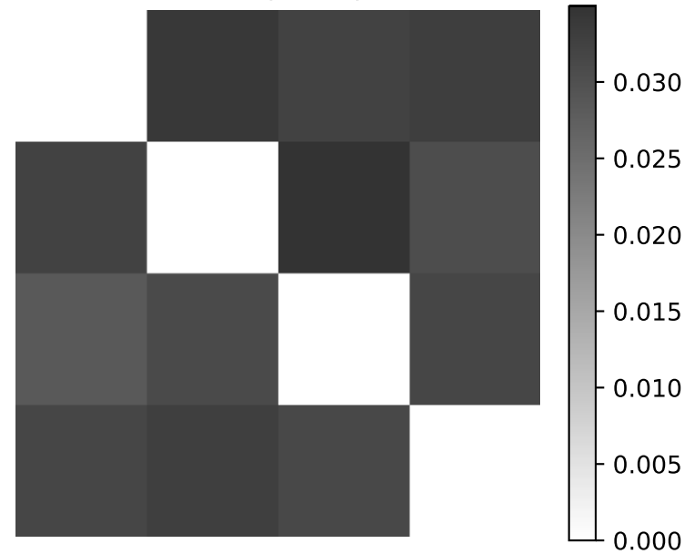
MAE (T=50)
