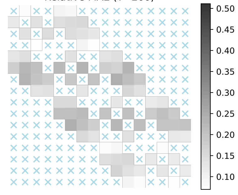
Relative MAE (T=200)
