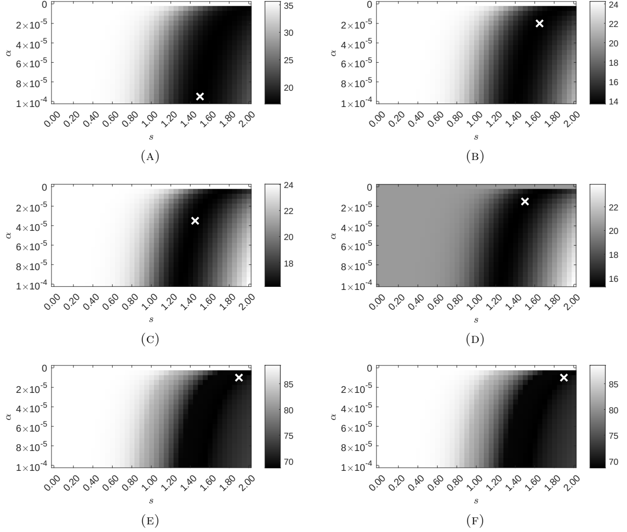
FIGURE S9. f/cFTBP reconstruction errors as functions of the regularization parameters \alpha and s for the rotated flag phantom, without (left column) and with (right column) the positivity constraint. Rows correspond to the L^1 , L^2 , and L^\infty error metrics.
