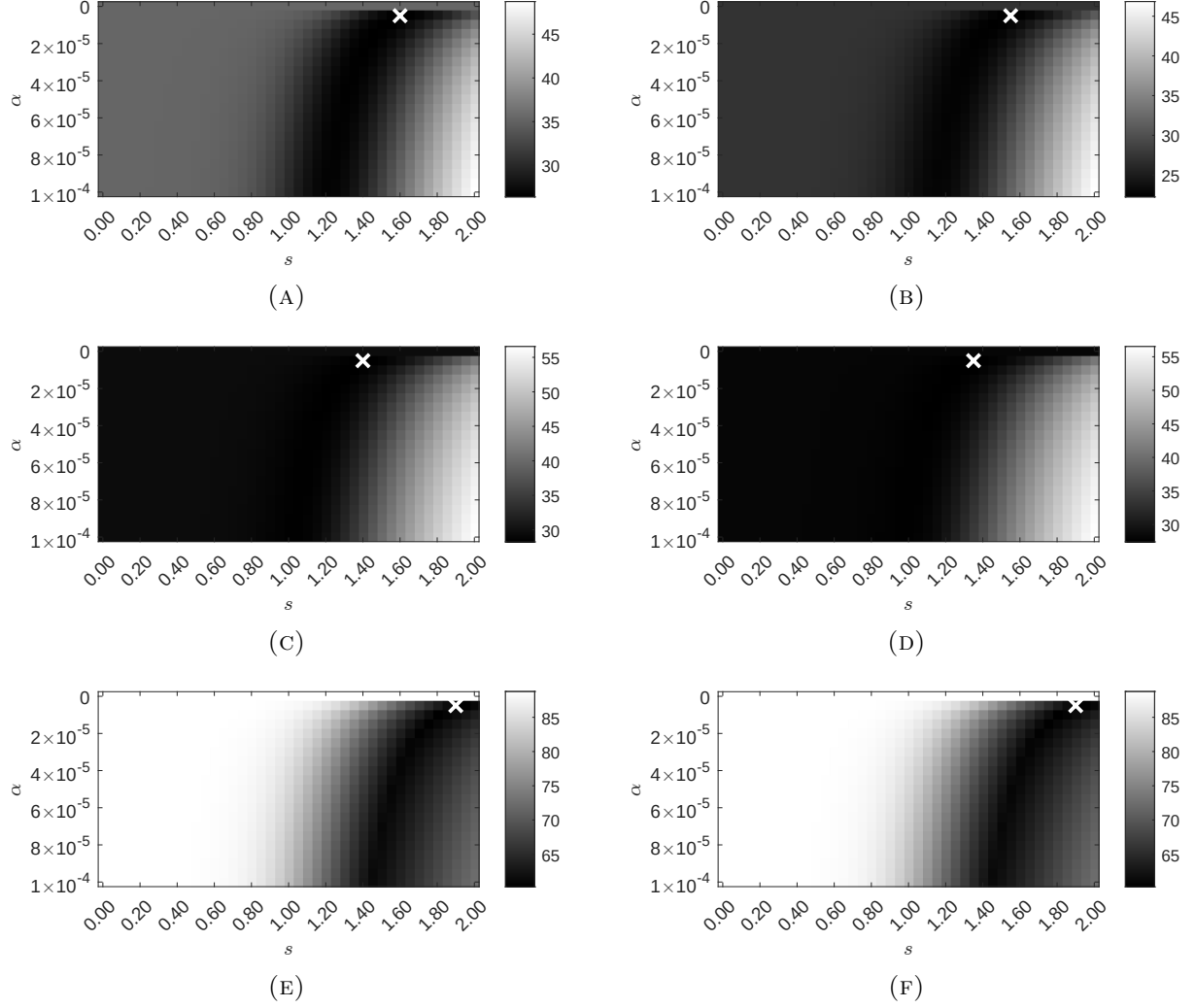
FIGURE S7. f/cFTBP reconstruction errors as functions of the regularization parameters \alpha and s for the Shepp–Logan phantom, without (left column) and with (right column) the positivity constraint. Rows correspond to the L^1 , L^2 , and L^\infty error metrics.
