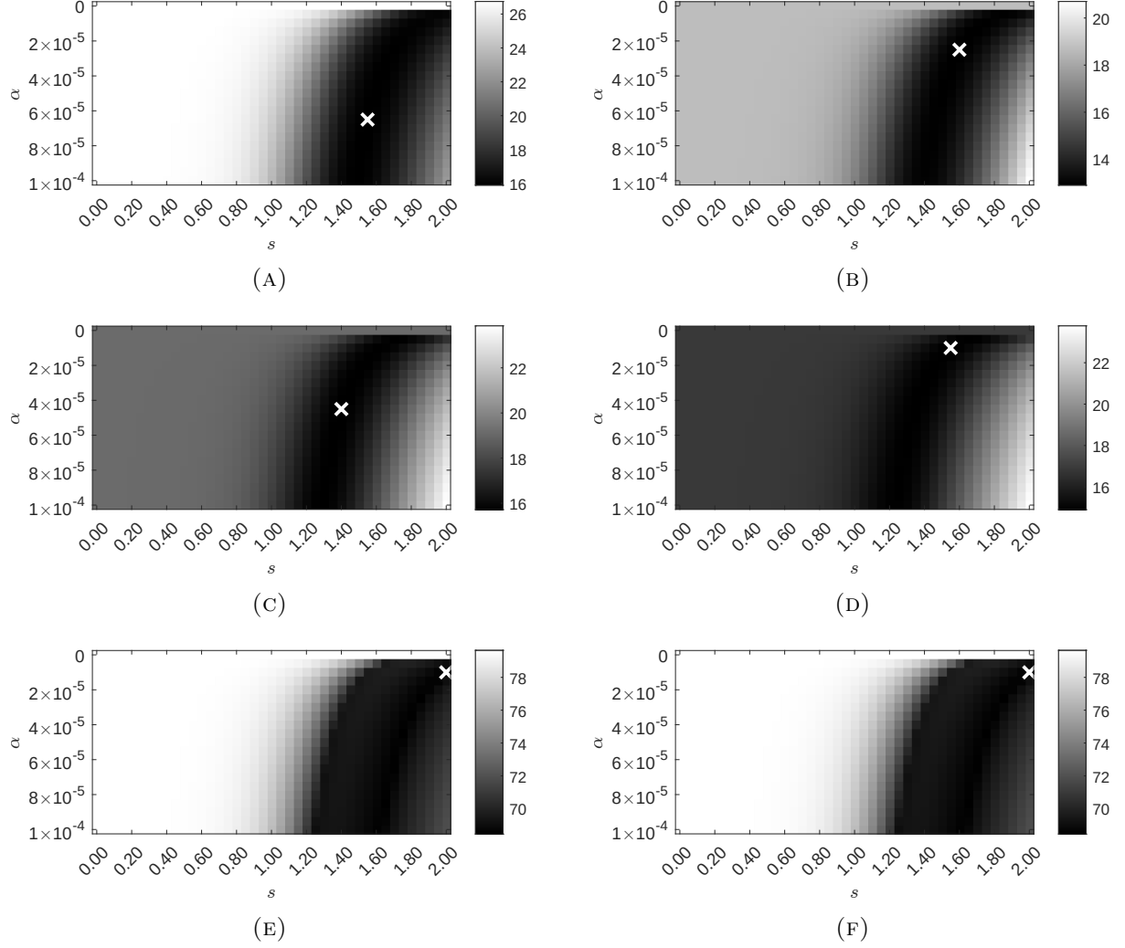
FIGURE S3. Torus CT reconstruction errors as functions of the regularization parameters \alpha and s for the rotated flag phantom, without (left column) and with (right column) the positivity constraint. Rows correspond to the L^1 , L^2 , and L^\infty error metrics.
