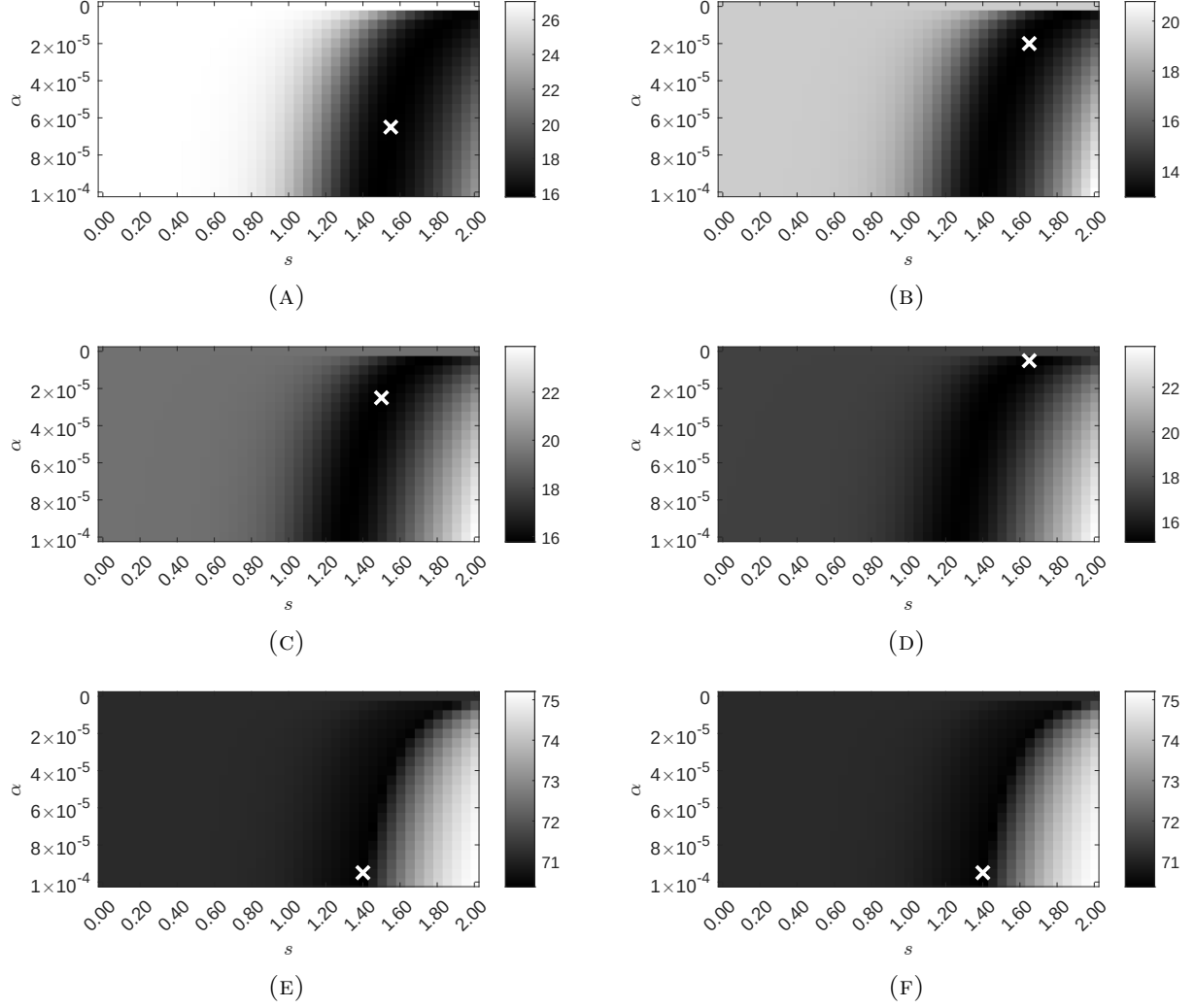
FIGURE S2. Torus CT reconstruction errors as functions of the regularization parameters \alpha and s for the flag phantom, without (left column) and with (right column) the positivity constraint. Rows correspond to the L^1 , L^2 , and L^\infty error metrics.
