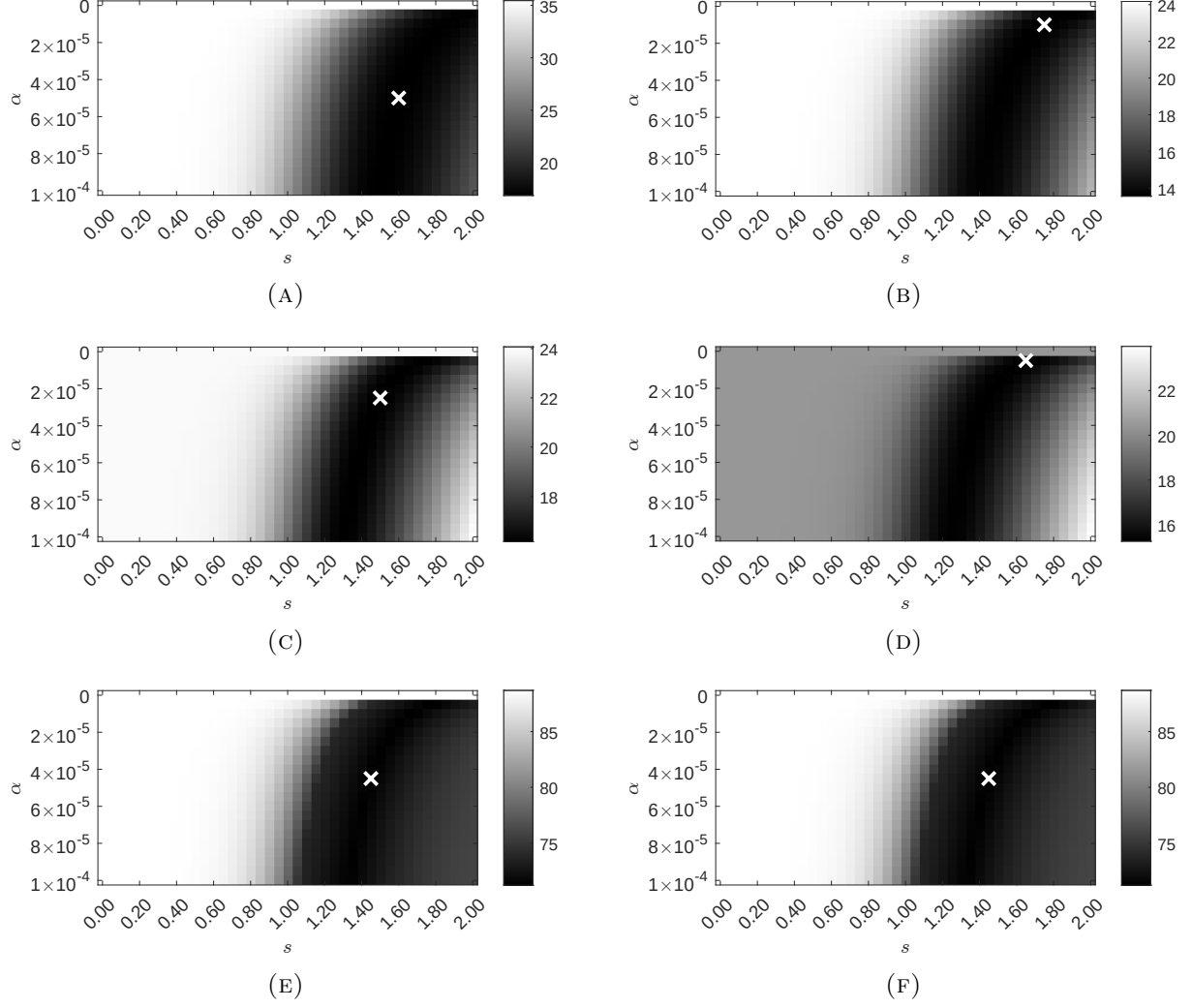
FIGURE S8. f/cFTBP reconstruction errors as functions of the regularization parameters \alpha and s for the flag phantom, without (left column) and with (right column) the positivity constraint. Rows correspond to the L^1 , L^2 , and L^\infty error metrics.
