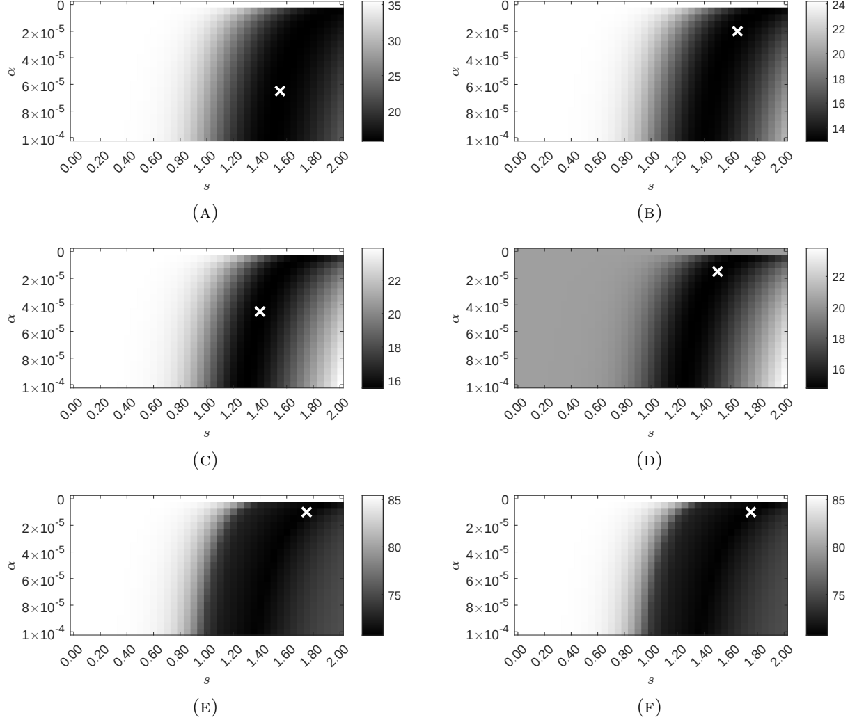
FIGURE S5. Star TCT reconstruction errors as functions of the regularization parameters \alpha and s for the flag phantom, without (left column) and with (right column) the positivity constraint. Rows correspond to the L^1 , L^2 , and L^\infty error metrics.
