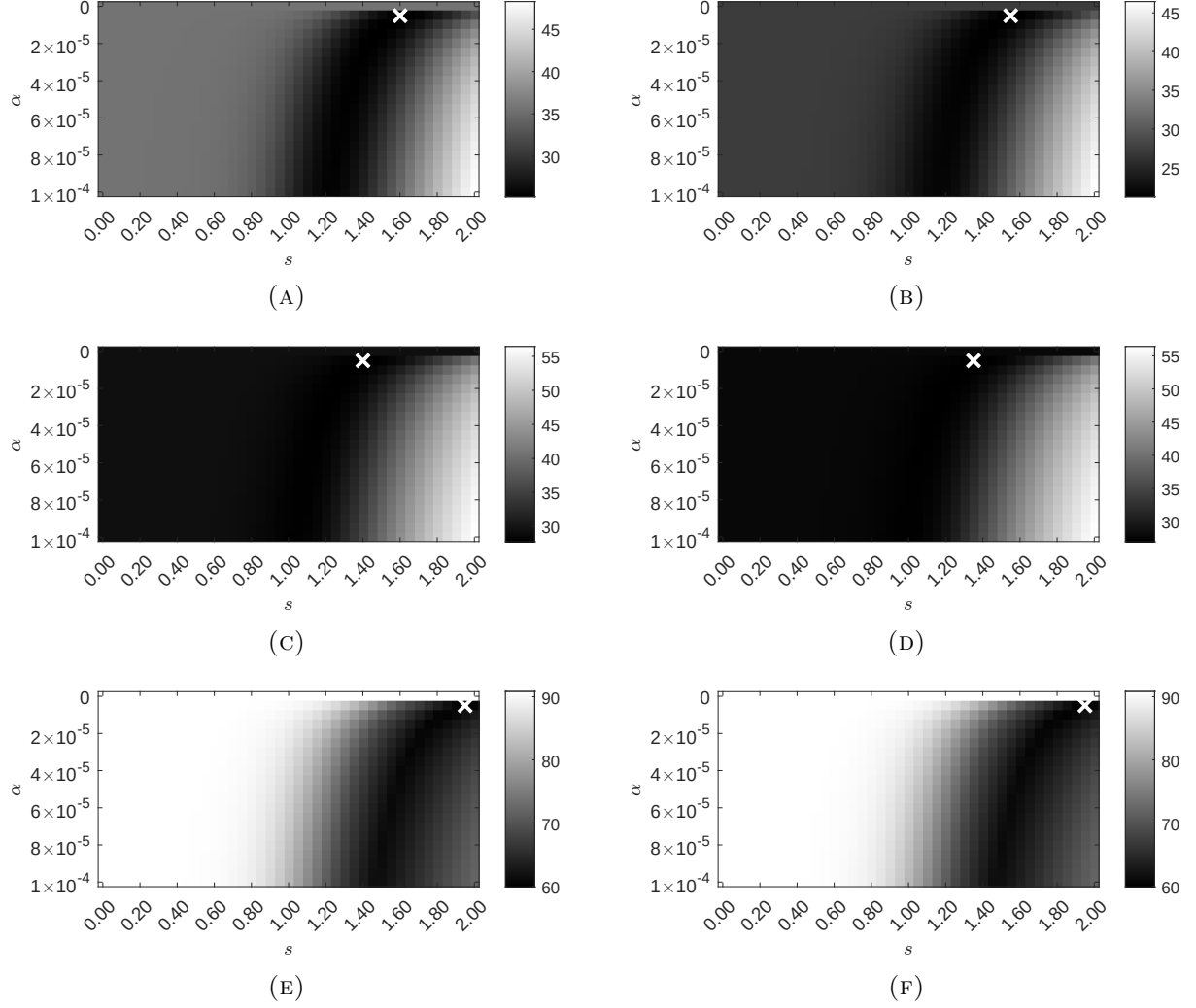
FIGURE S4. Star TCT reconstruction errors as functions of the regularization parameters \alpha and s for the Shepp–Logan phantom, without (left column) and with (right column) the positivity constraint. Rows correspond to the L^1 , L^2 , and L^\infty error metrics.
