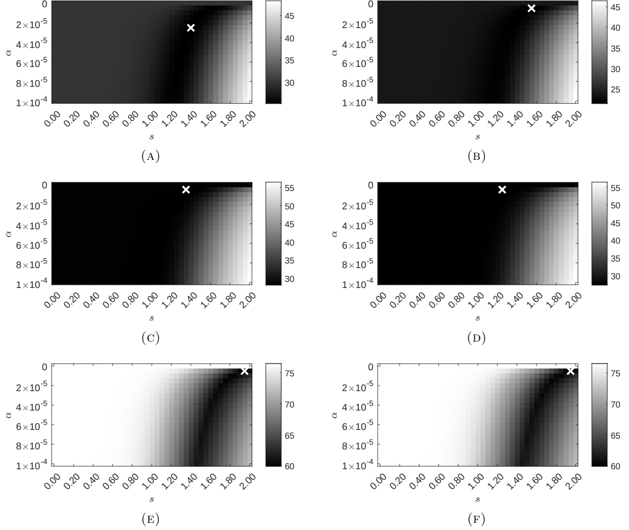
FIGURE S1. Torus CT reconstruction errors as functions of the regularization parameters \alpha and s for the Shepp–Logan phantom, without (left column) and with (right column) the positivity constraint. Rows correspond to the L^1 , L^2 , and L^\infty error metrics.
