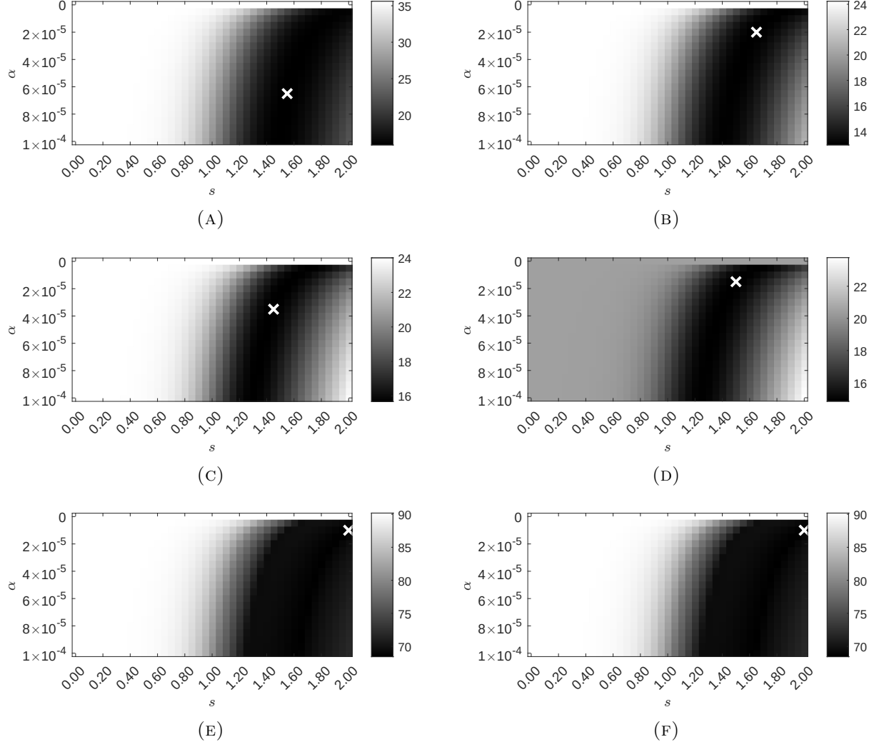
FIGURE S6. Star TCT reconstruction errors as functions of the regularization parameters \alpha and s for the rotated flag phantom, without (left column) and with (right column) the positivity constraint. Rows correspond to the L^1 , L^2 , and L^\infty error metrics.
