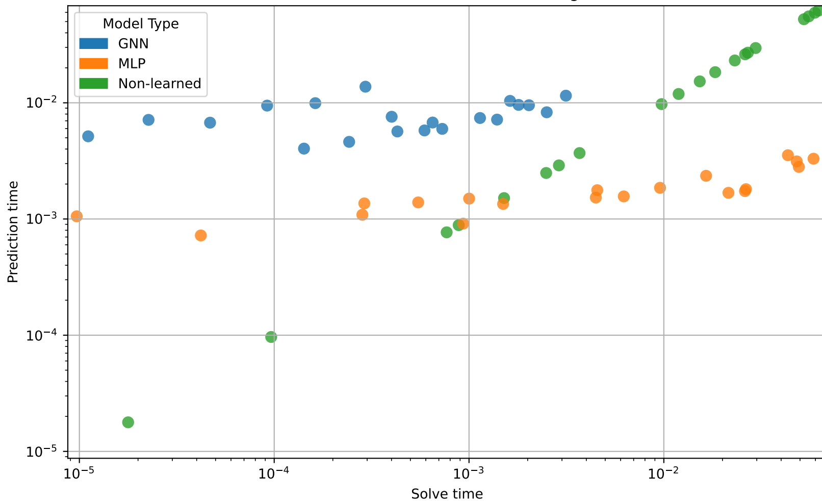
Prediction vs Solve Time with scaling size
