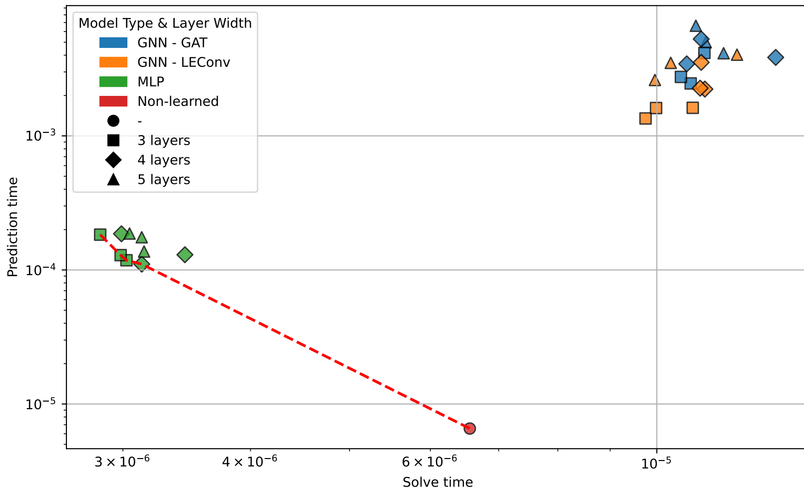
Prediction vs Solve Time (Pareto Front)
