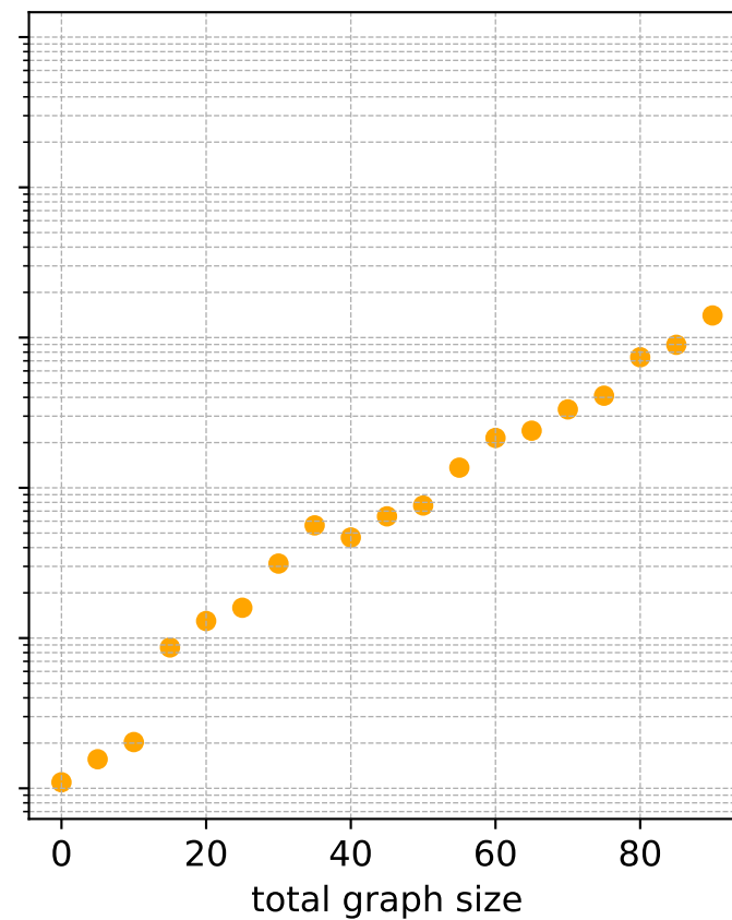
Non-learned
