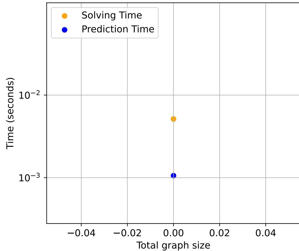
GNN
