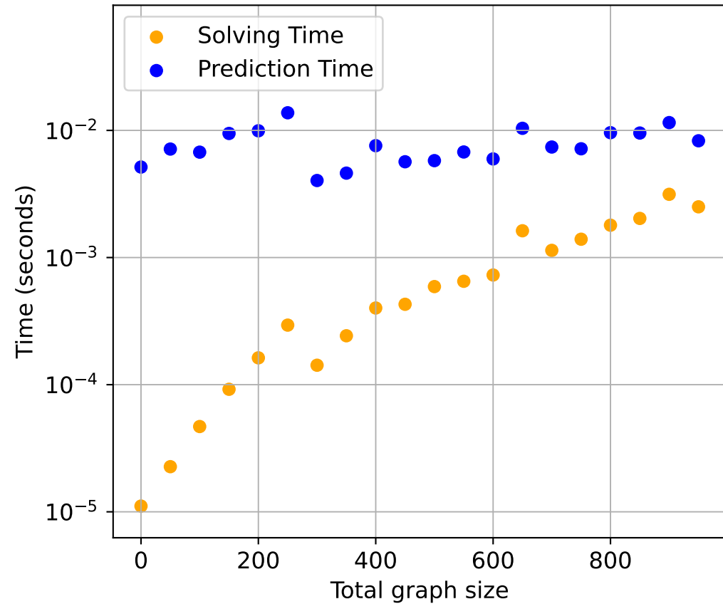
GNN
