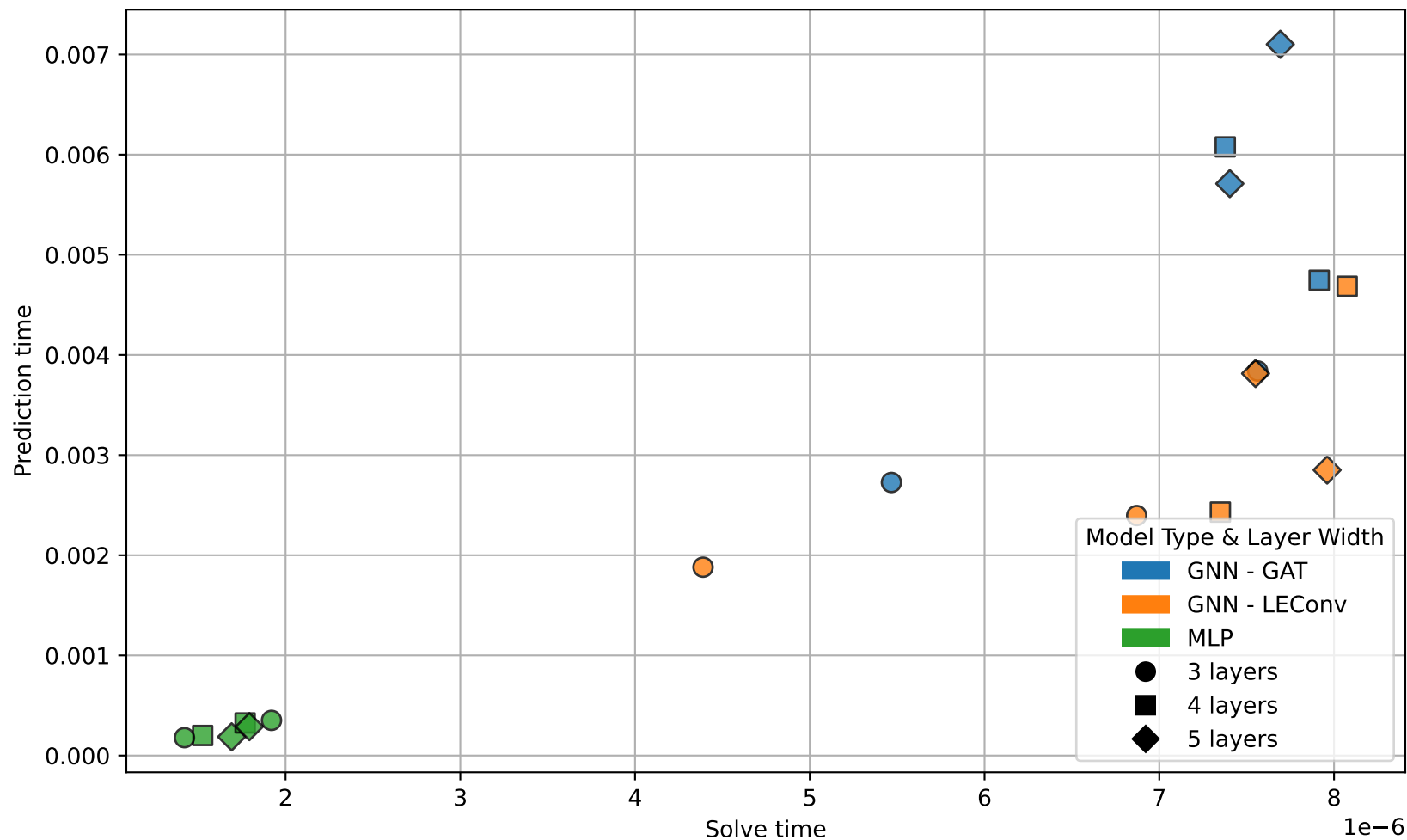
Prediction vs Solve Time (Pareto Front)
