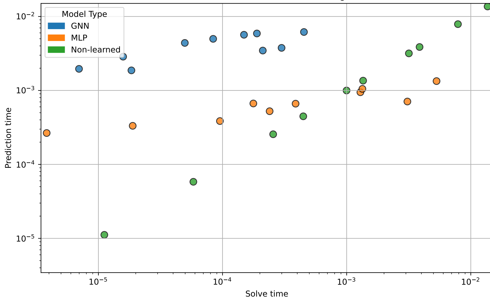
Prediction vs Solve Time with sclaing size
