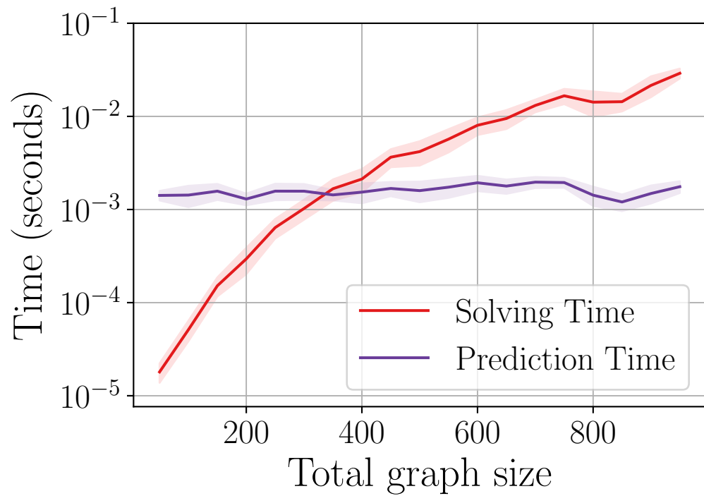
(a) GNN
