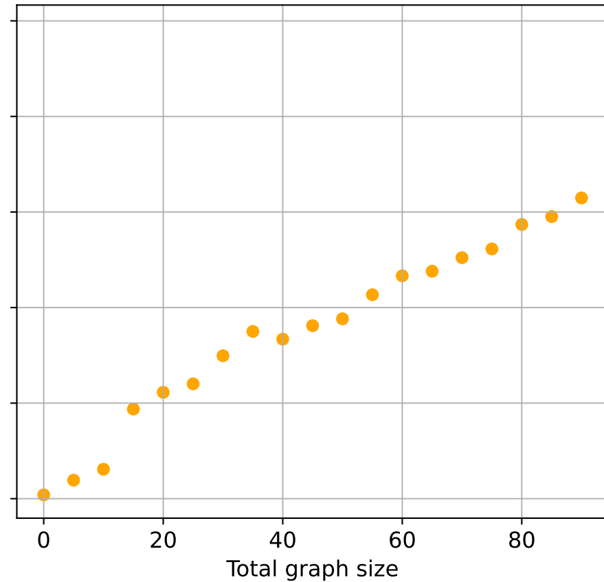
Non-learned
