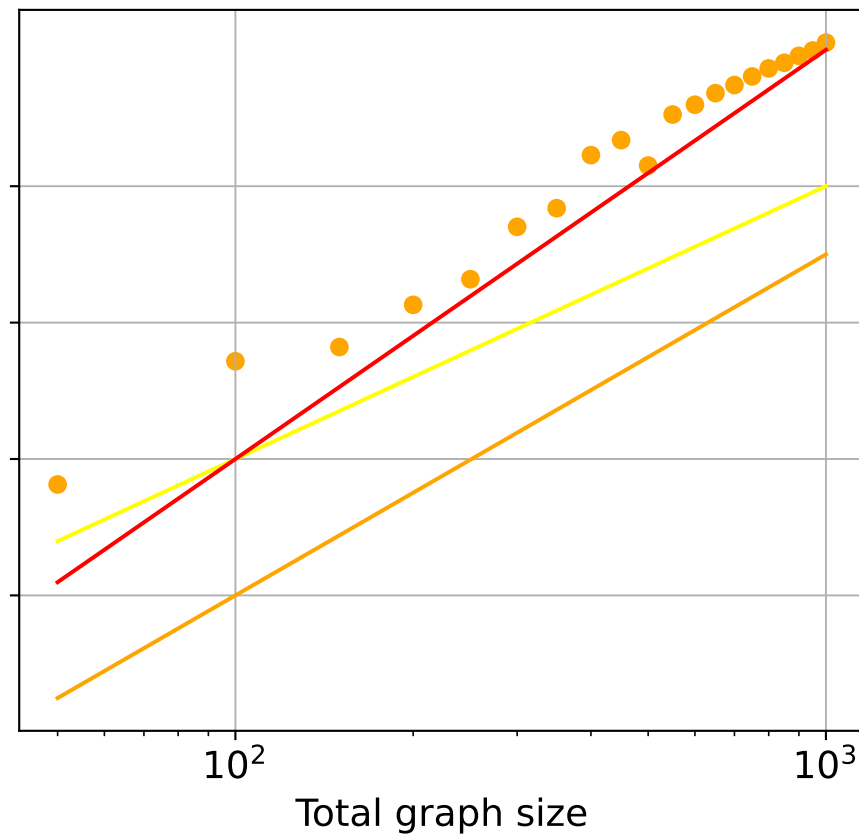
Non-learned
