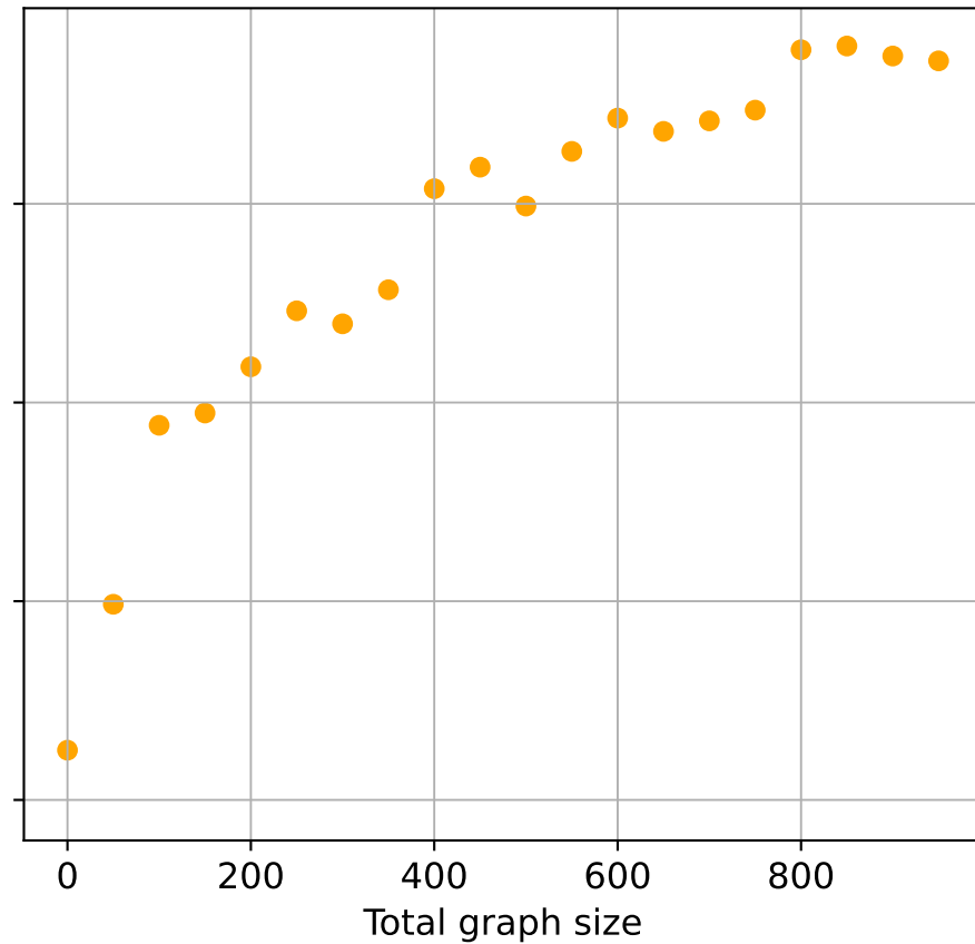
Non-learned
