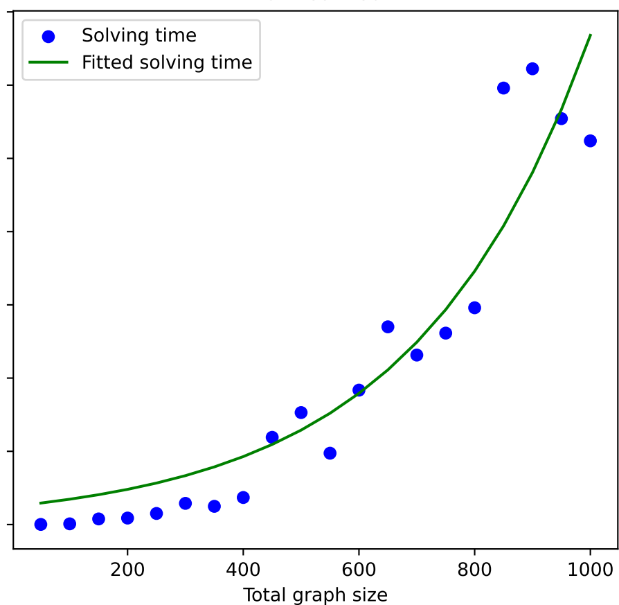
Non-learned
