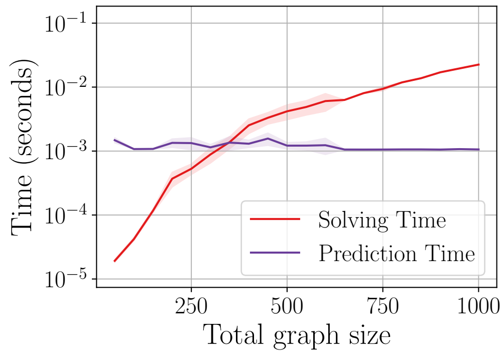
(a) GNN
