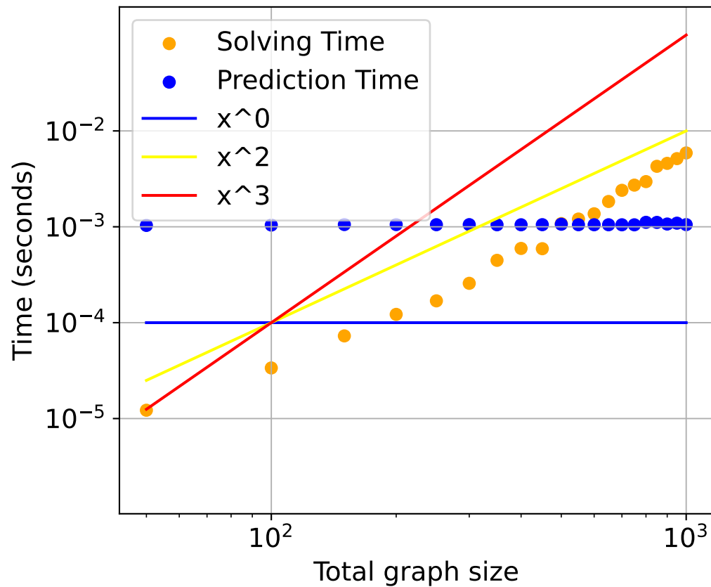
GNN
