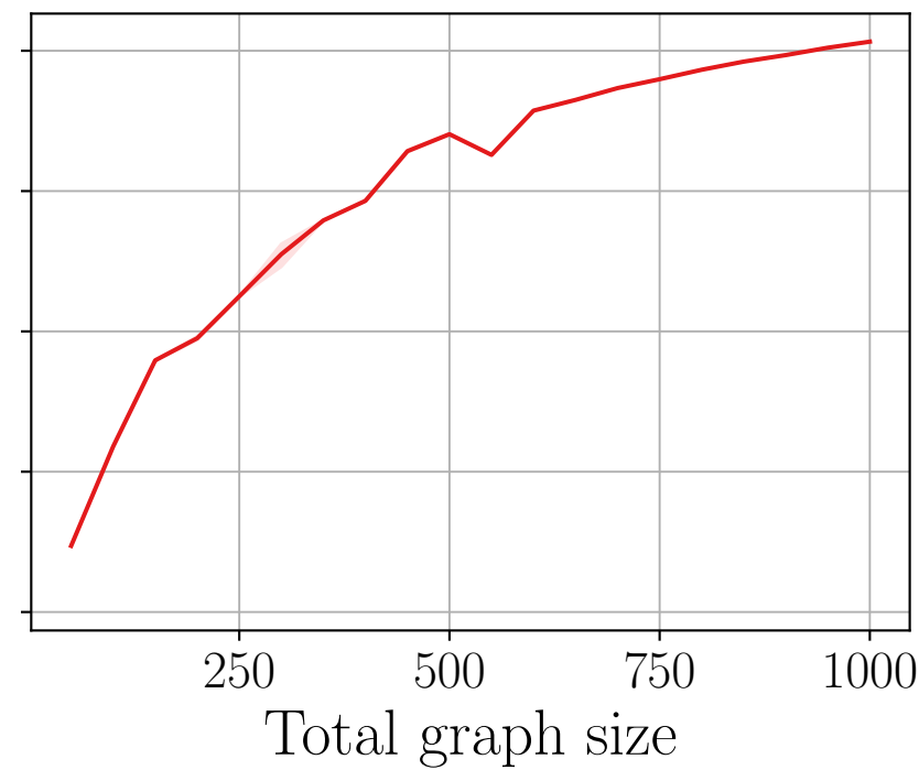
(c) Non-learned
