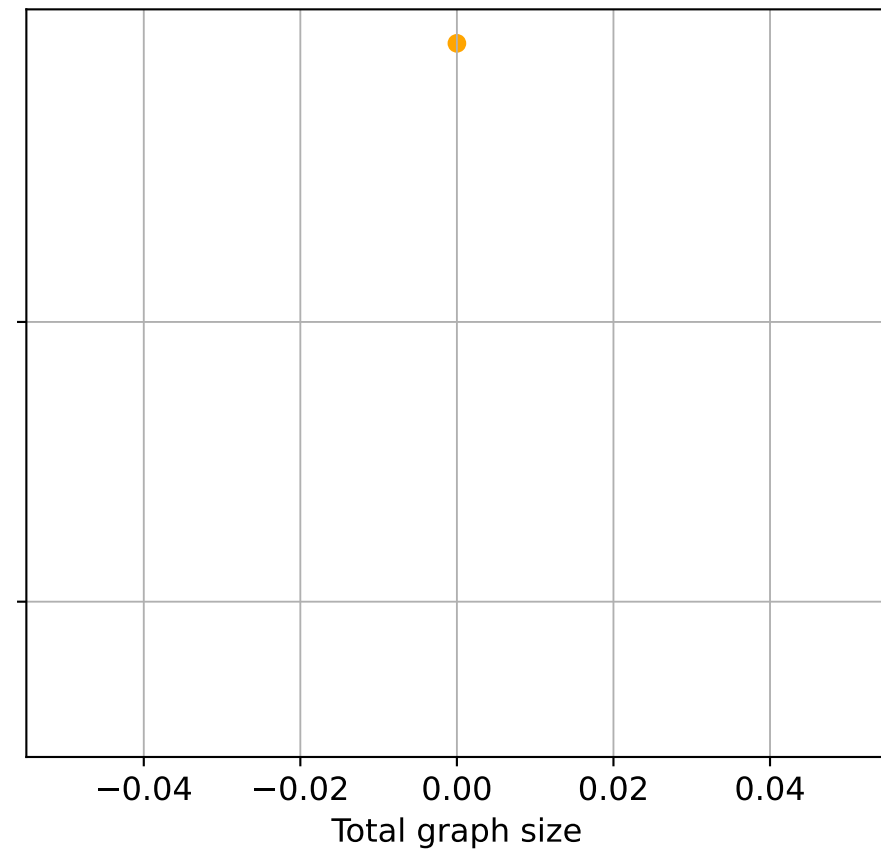
Non-learned
