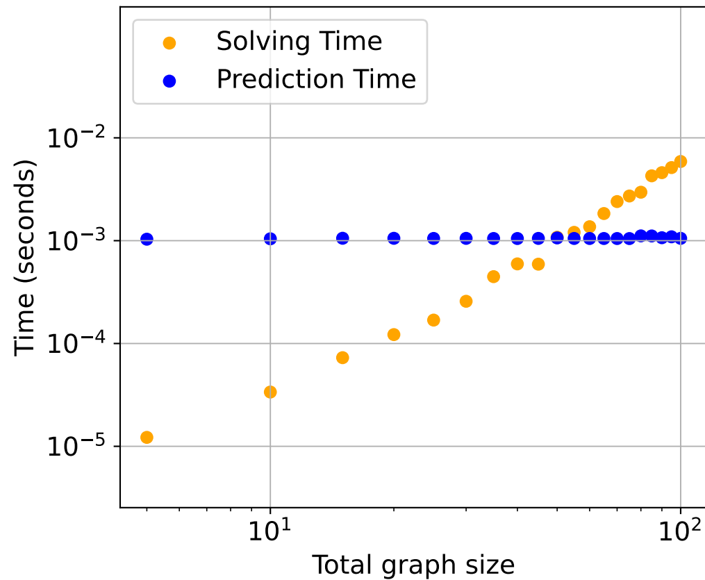
GNN
