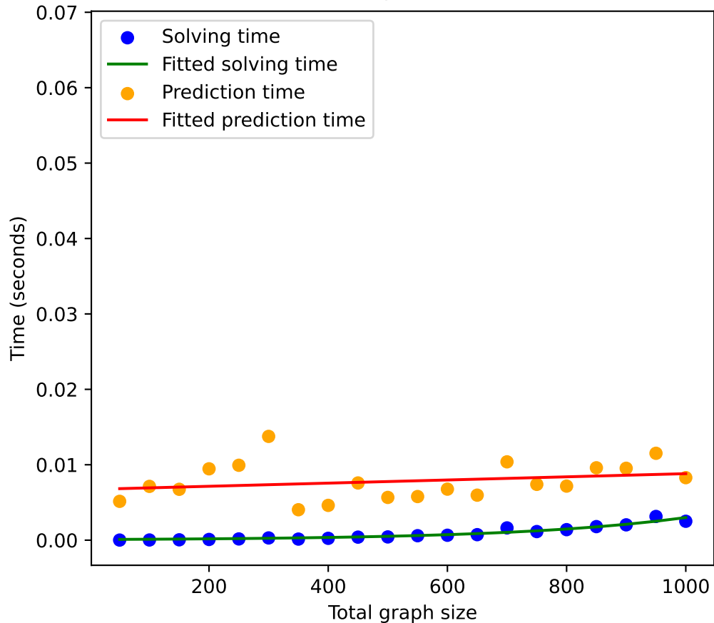
GNN
