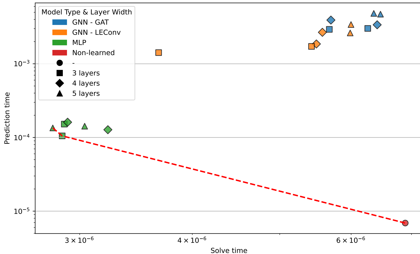
Prediction vs Solve Time (Pareto Front)
