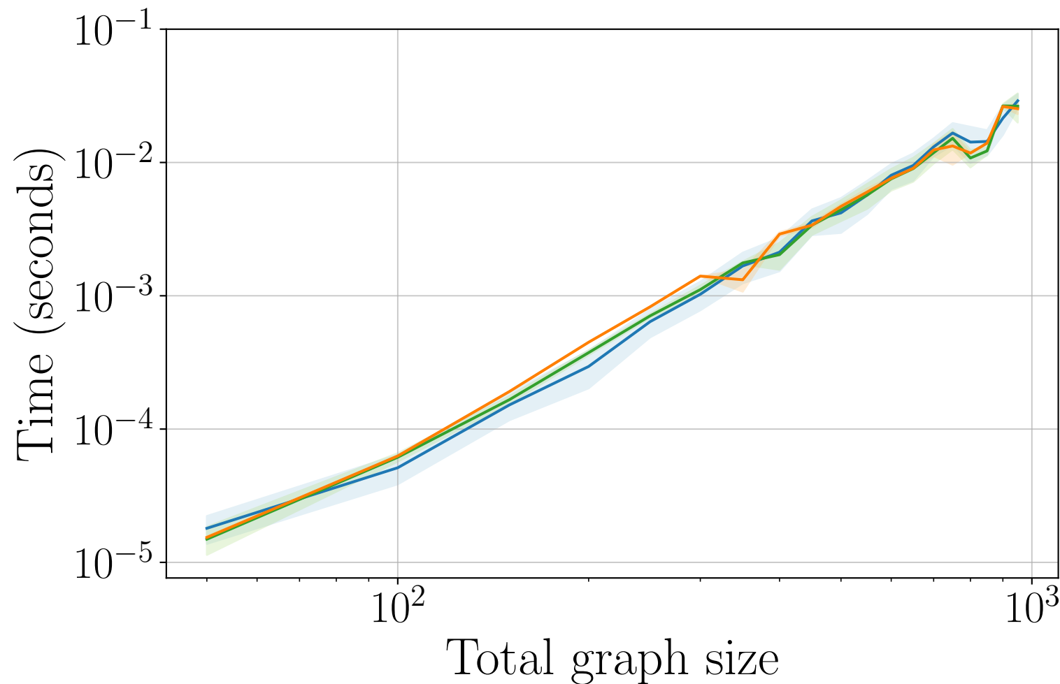
(a) Solve time
