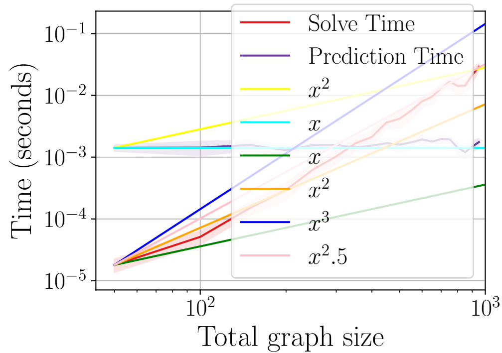
(a) GNN
