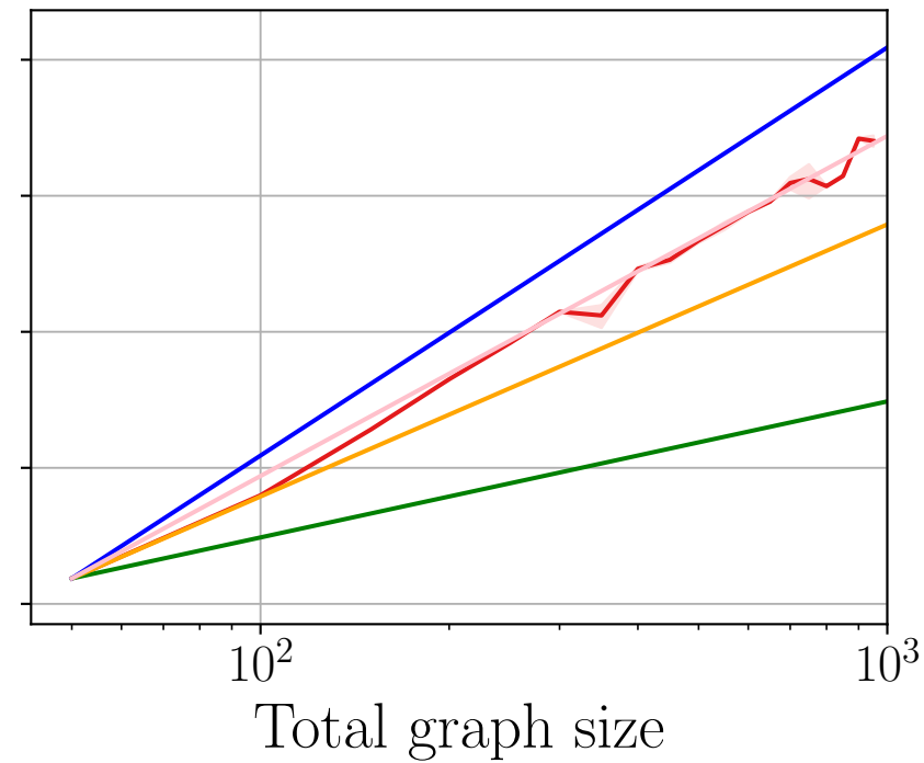
(c) Cold-started
