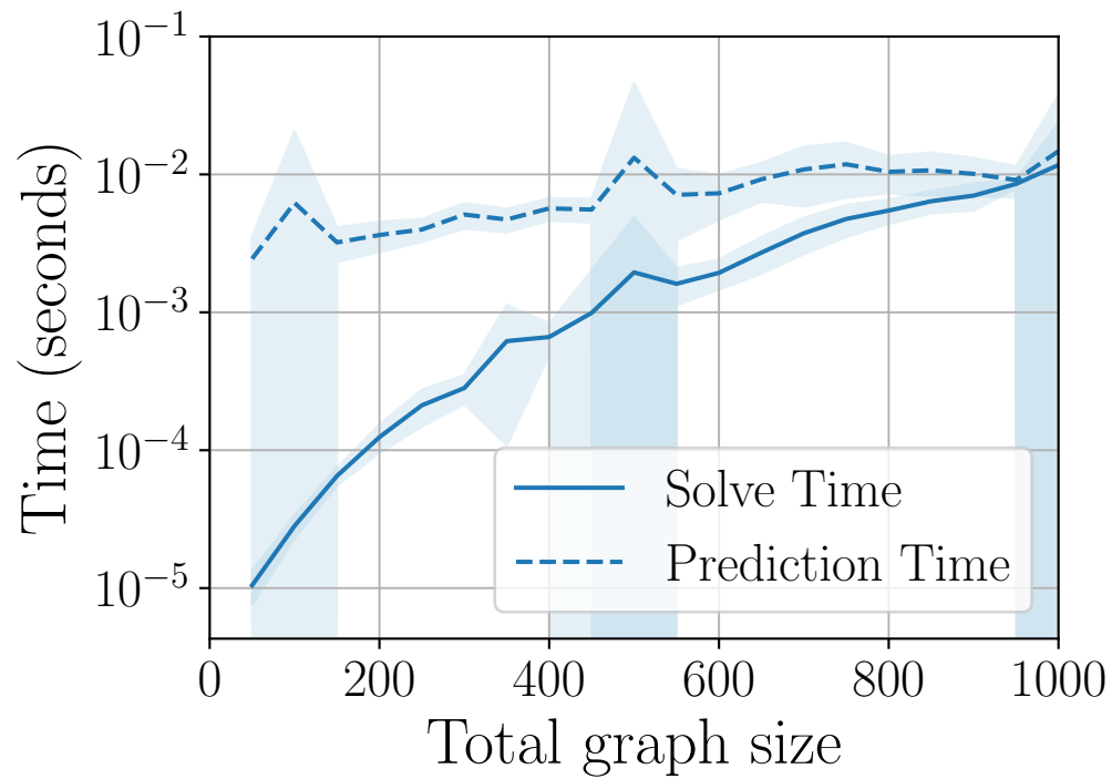
(a) GNN
