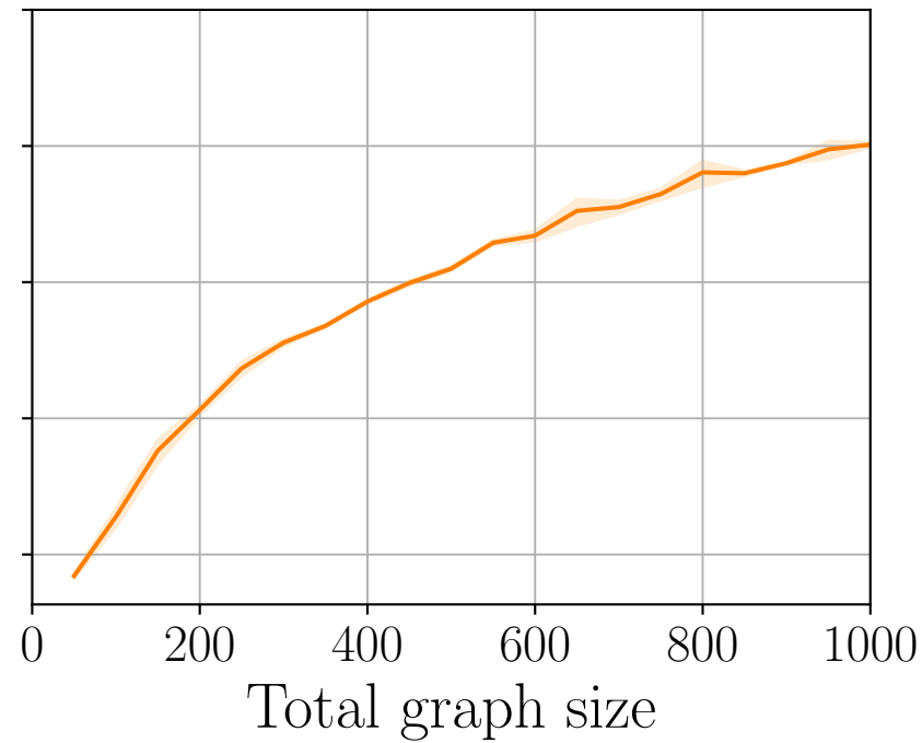
(c) Cold-started
