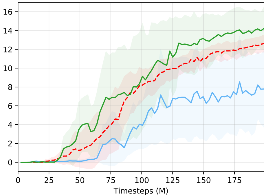
Number of Baoding rotations (minimal, no bad seeds)
