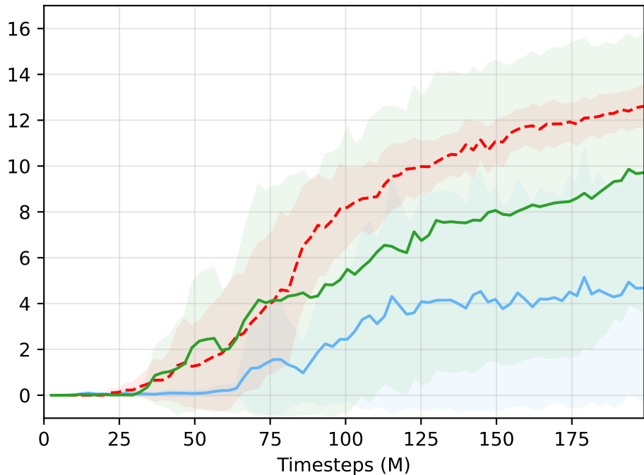
Number of Baoding rotations (minimal, all seeds)
