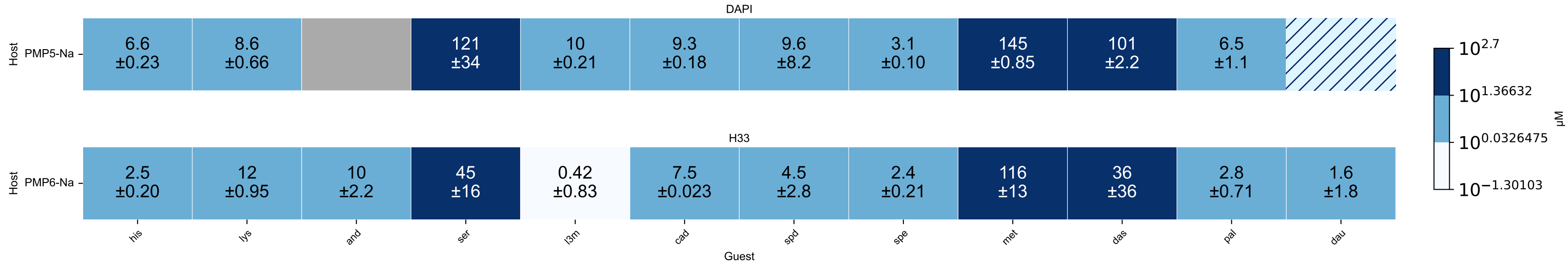
Competition Binding — K_i (by Dye) (page 1)
