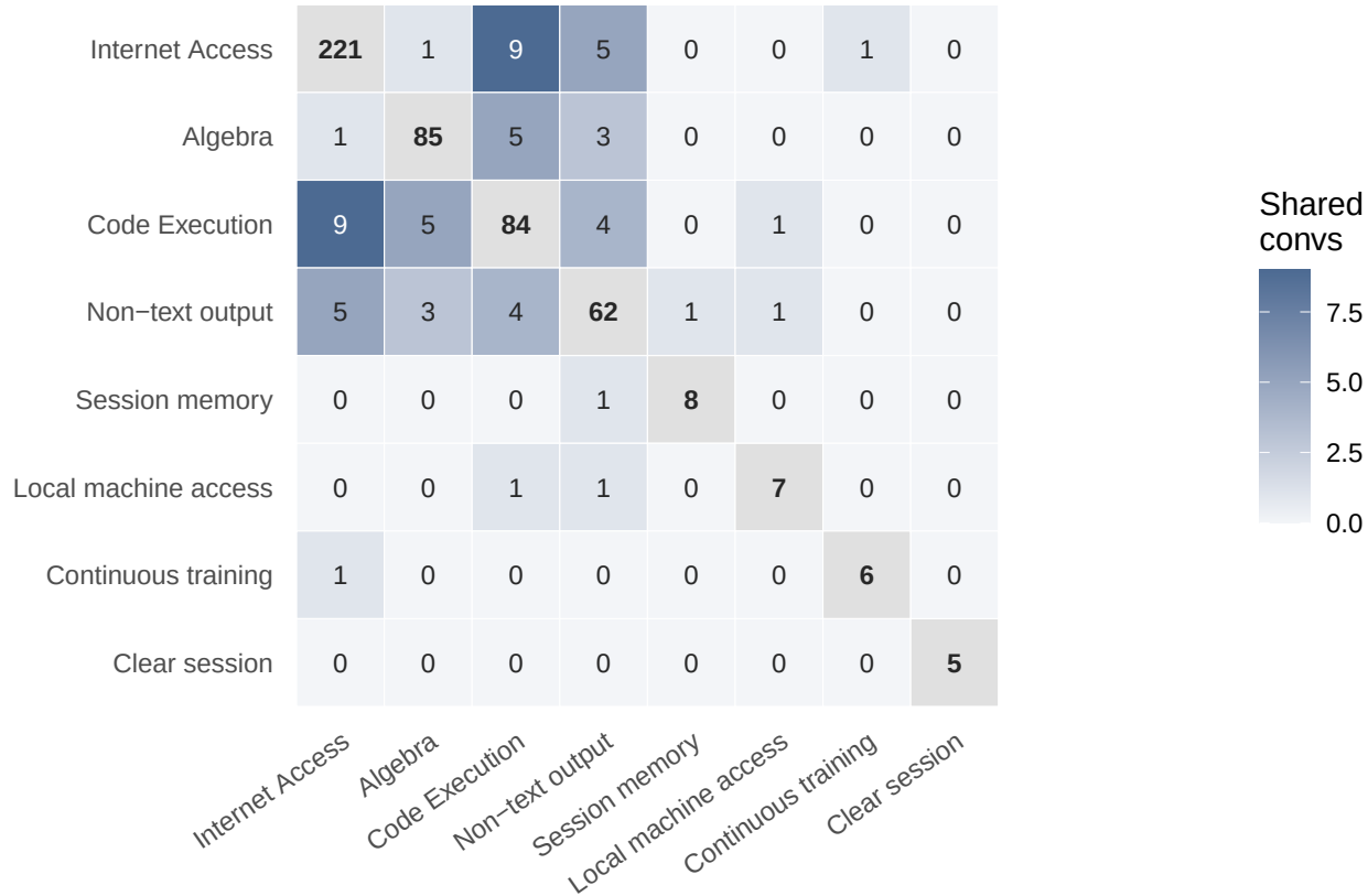
(b) Pairwise co-occurrence (diagonal = code total)
