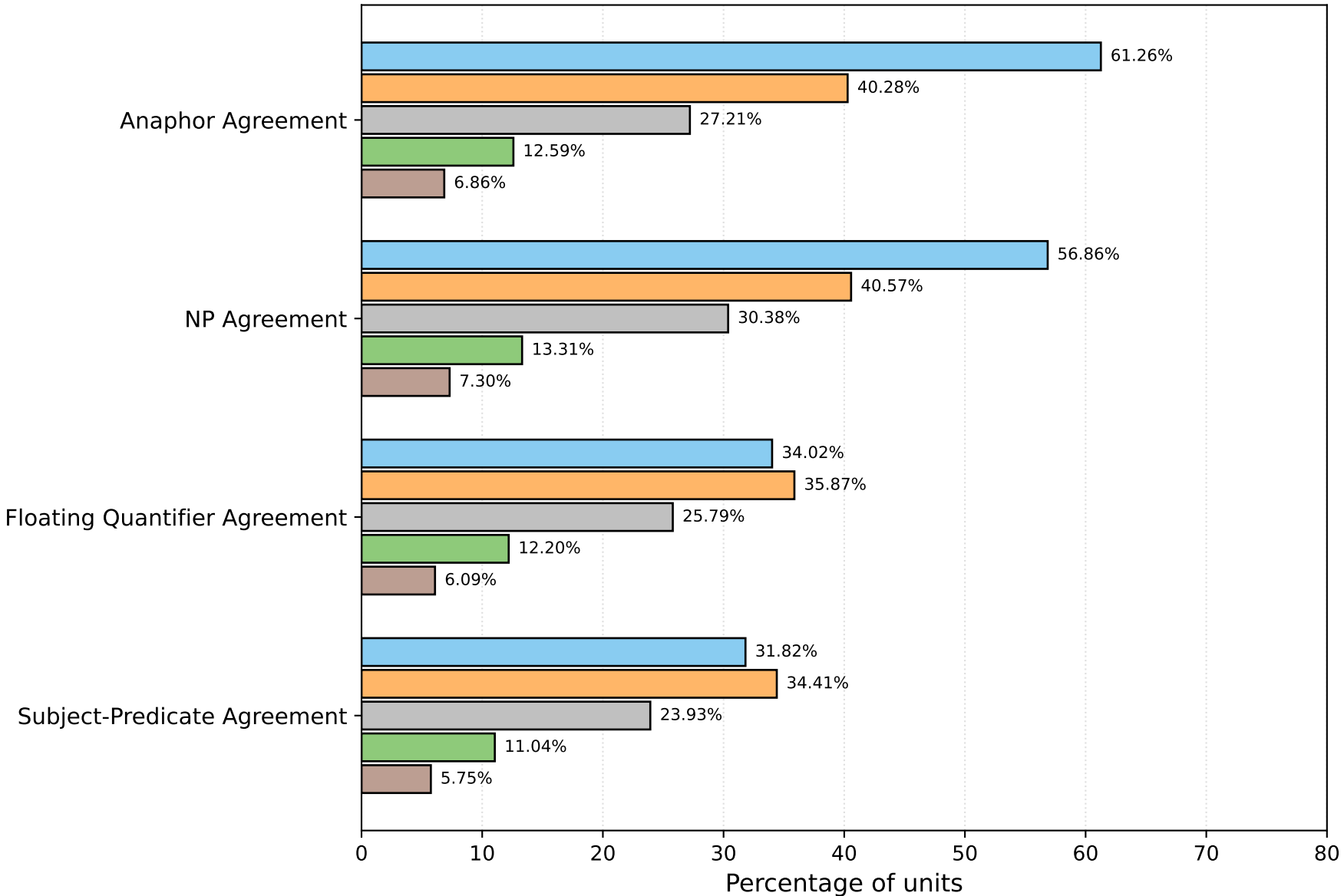
Cross-phenomenon overlap in RuBLiMP (agreement, gemma-3-4b-pt)
