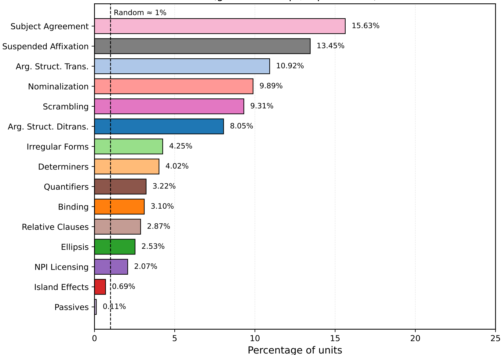
Overlap of Anaphor Agreement with other TurBLiMP phenomena (gemma-3-4b-pt, top 1% units)
