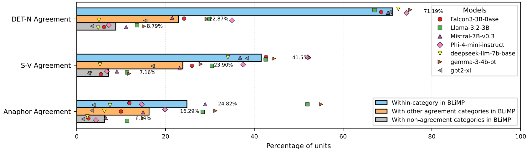
Agreement overlap in BLiMP across seven models
