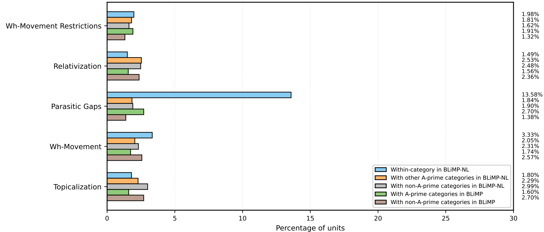
Cross-phenomenon overlap in BLiMP-NL (A-prime dependencies)
