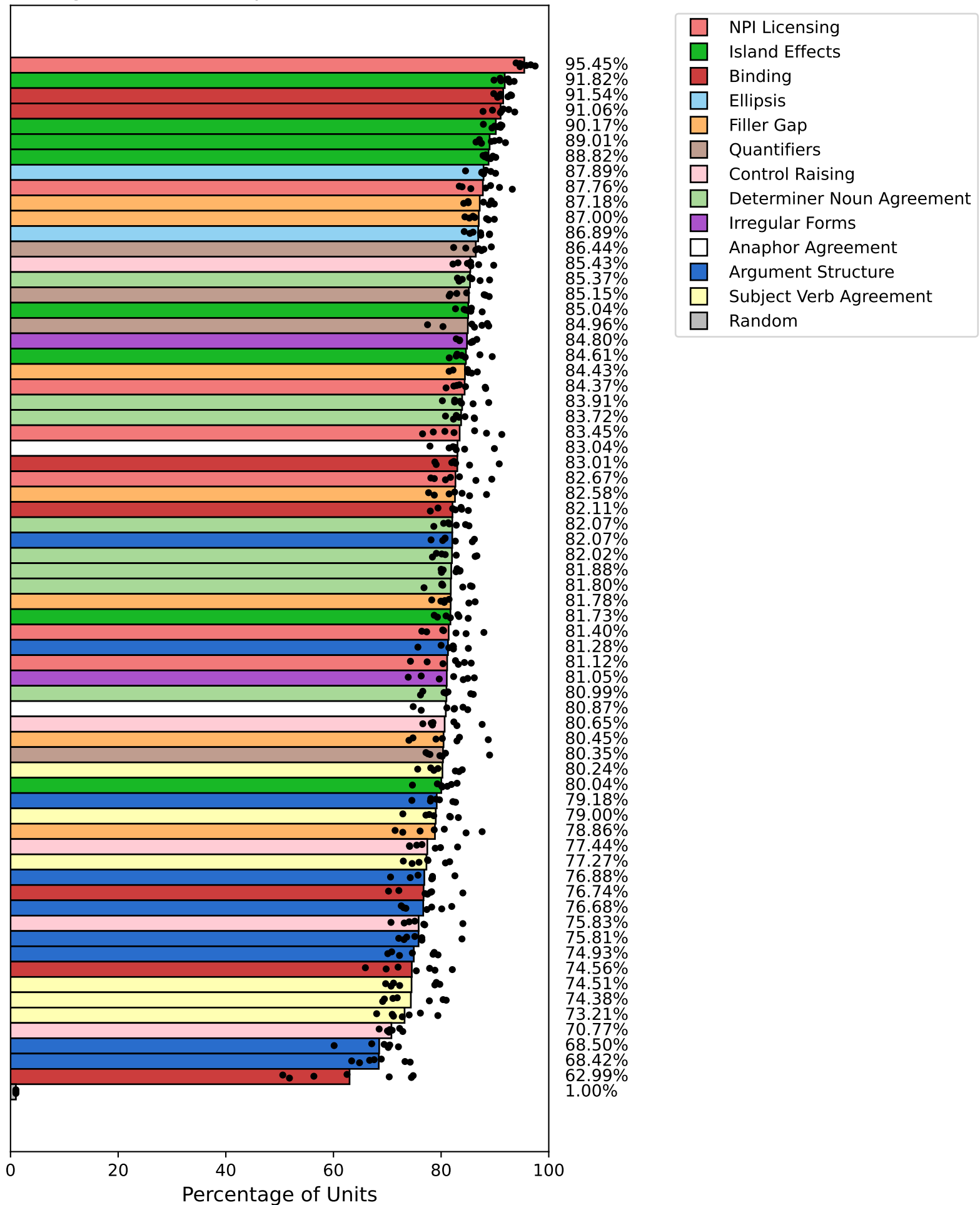
Average 2-fold overlap across models on BLiMP
