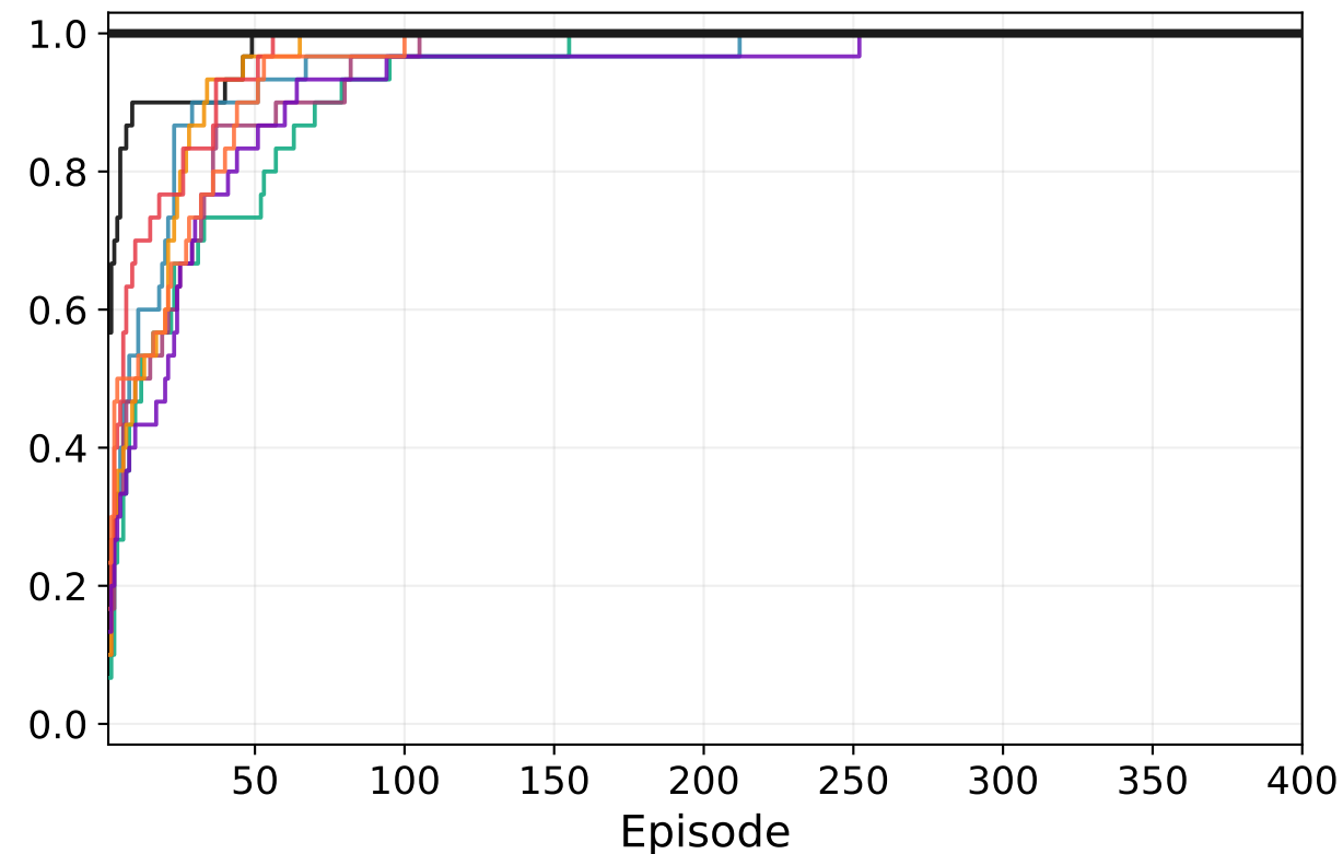
Pretrained
