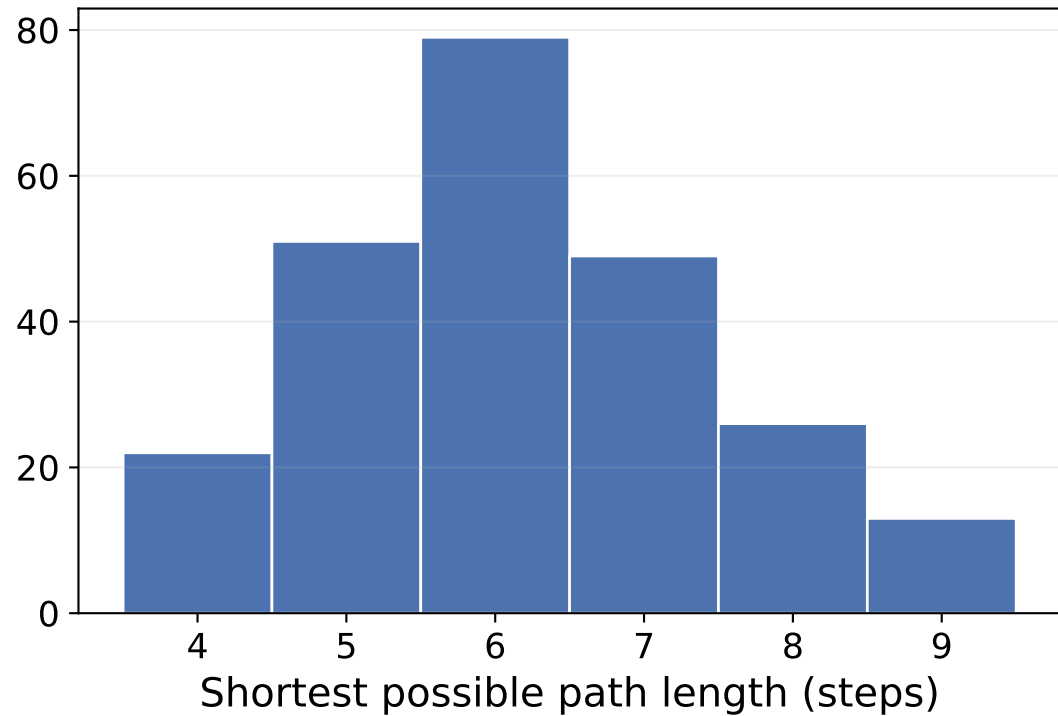
Pretrained (n=240, mean=6.19, sd=1.29)
