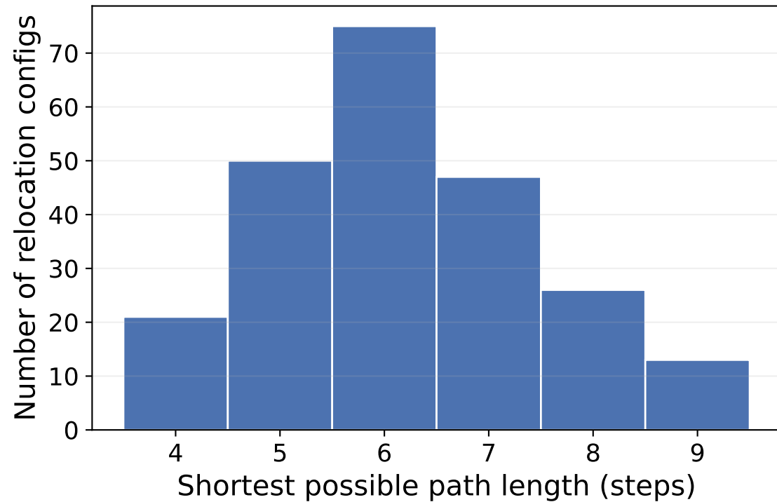
Cold Start (n=232, mean=6.20, sd=1.30)
