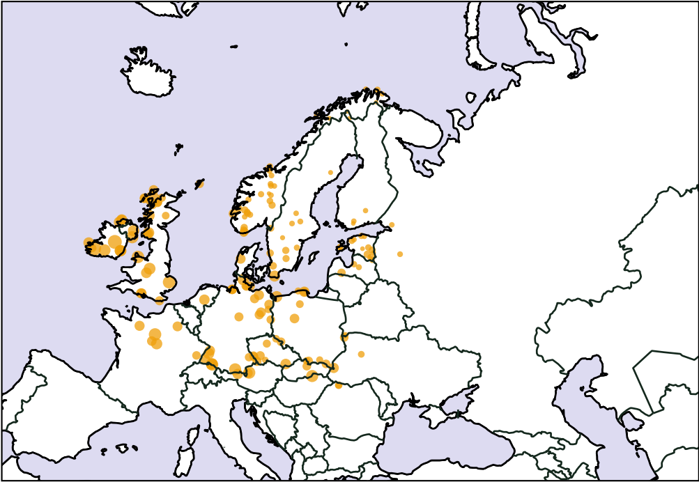
2000-0 BP
