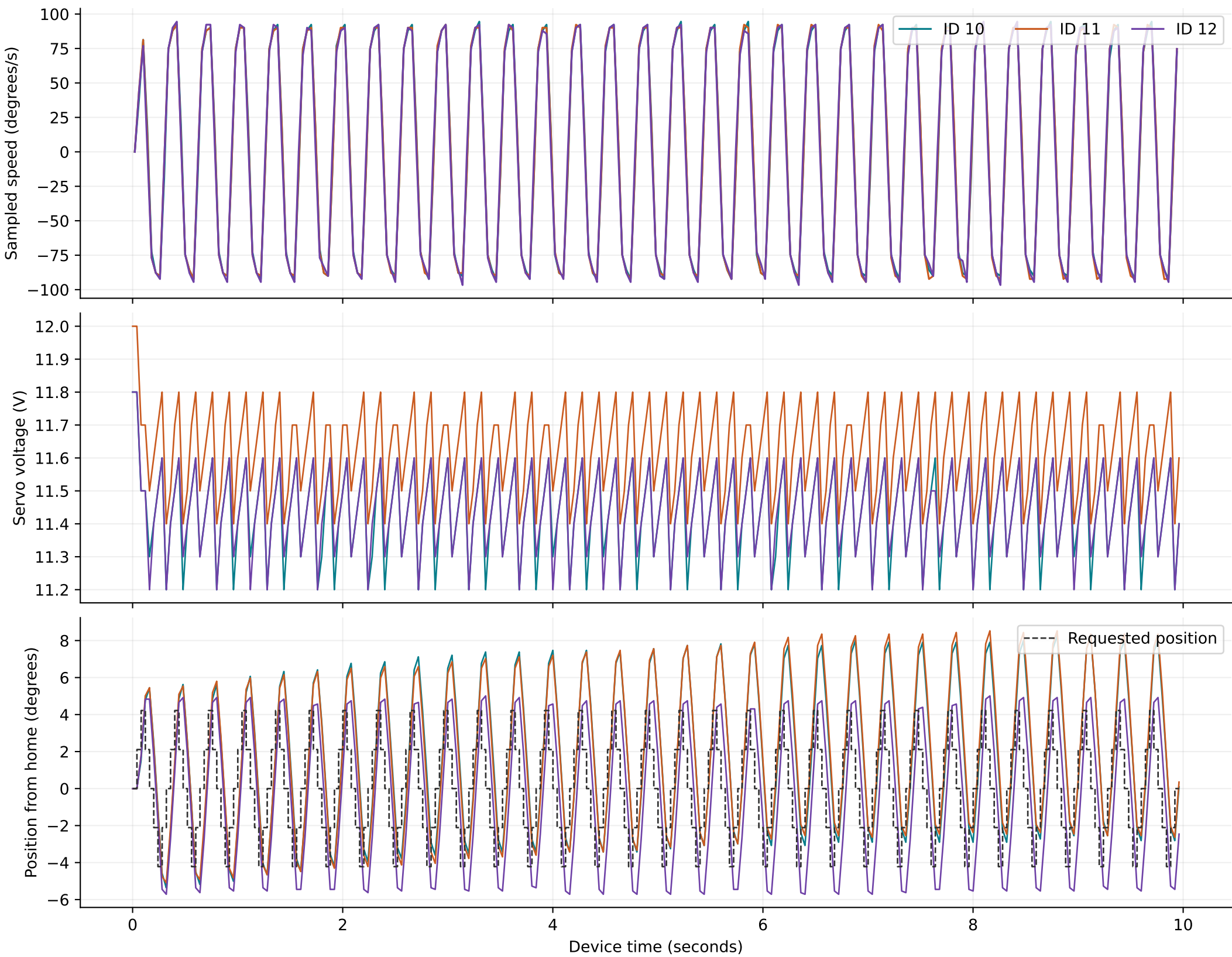
Three real motors — third 10-second reversal block at 35% drive 12 V supply setting; all stops verified; existing FPGA controller
