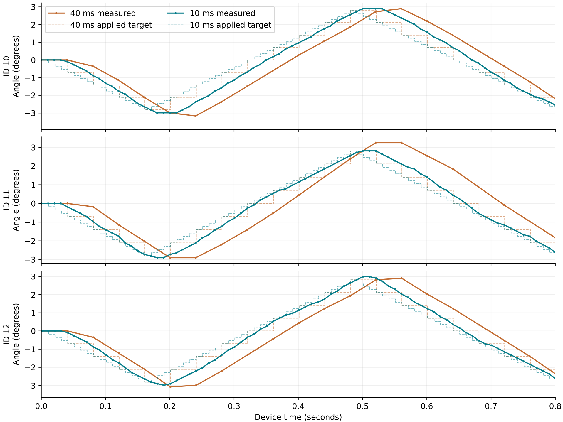
Real three-motor motion: 40 ms versus 10 ms at 10% drive First trial of each configuration; first 0.8 s shown; fixed gains unchanged
