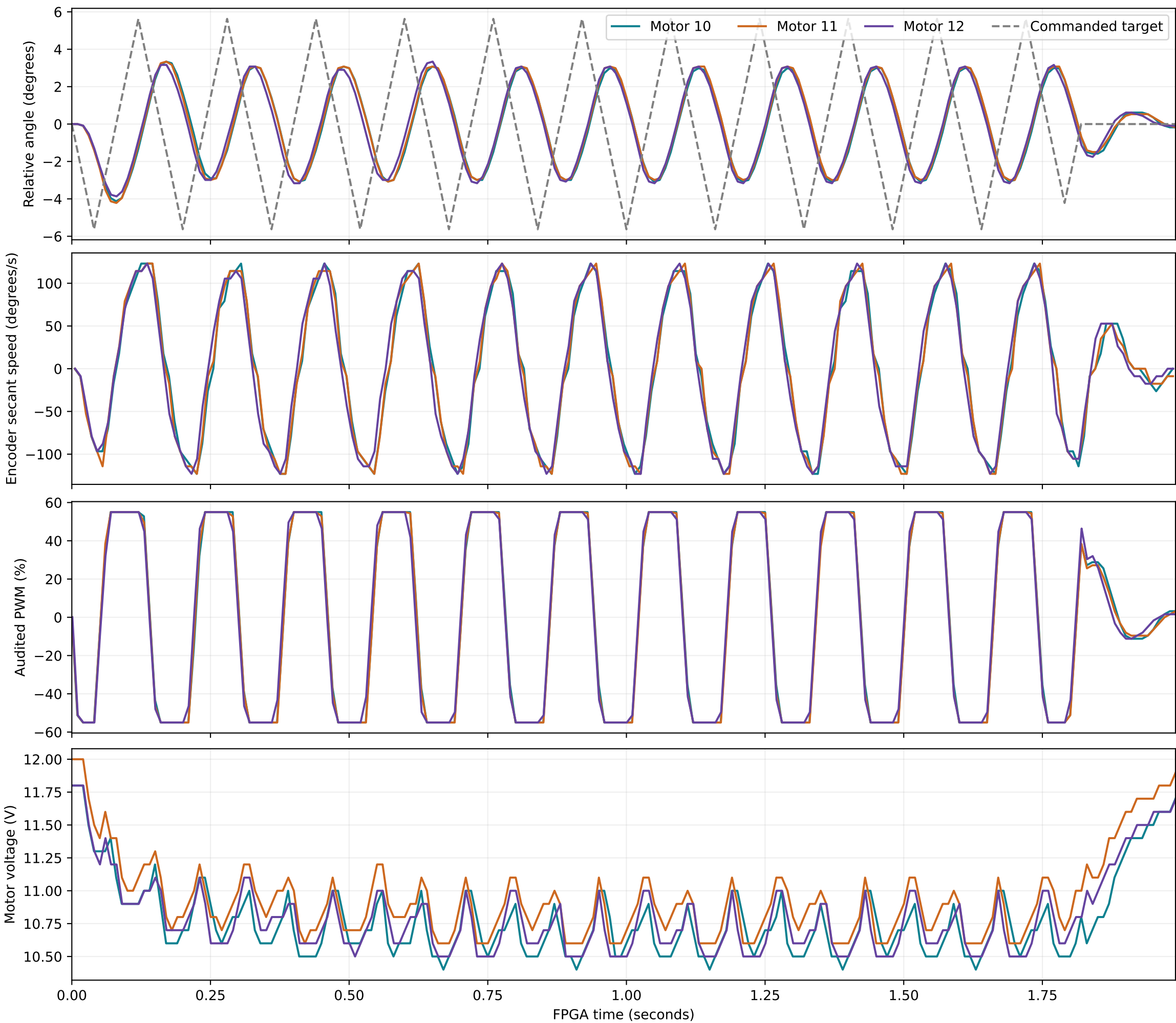
Three real motors at 100 Hz: 55% drive, repeated reversals Completed and stopped; 12.6% voltage sag ended drive escalation
