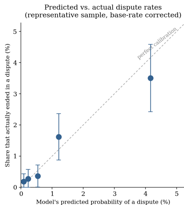
Figure 3: And its probabilities are honest. The same out-of-sample scores converted to real-world probabilities (per-platform base-rate correction), binned, against the share of markets that actually disputed; the dashed line is perfect calibration. When the model says \sim 4\% , about 3.5% of those markets blow up; every bin's CI crosses the line. The model doesn't just rank markets correctly — its numbers mean what they say.
