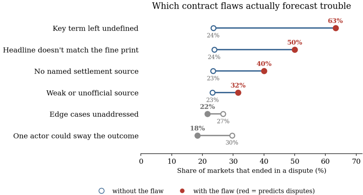
Figure 5: Which flaws carry the signal. Polymarket markets (organic disputes; n = 3,643 with 877 genuine specification disputes, dispute-enriched sample — levels are not real-world rates, the comparisons within each row are the point). Dispute rate without \rightarrow with each flaw: undefined key terms, headline/fine-print mismatch, and unnamed or weak settlement sources forecast trouble. In gray, the two that don't: edge-case coverage, and manipulability, which reverses — markets one actor could sway tend to resolve unambiguously and are disputed less. (Kalshi's exchange flags behave differently and are analyzed separately in the paper.)
