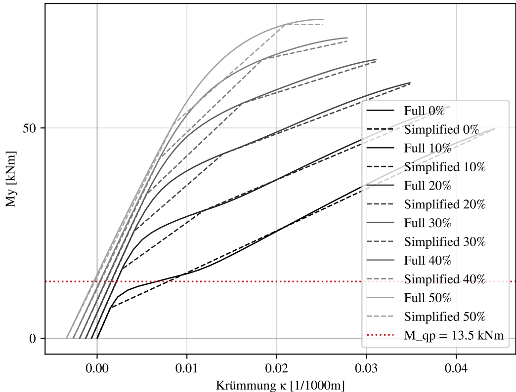
M-K-Diagrams at x_{\text{norm}} = 0.062 of C1_1 — full vs. simplified, varying prestress
