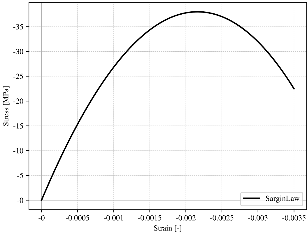
Constitutive Law of C30/37 SLS
