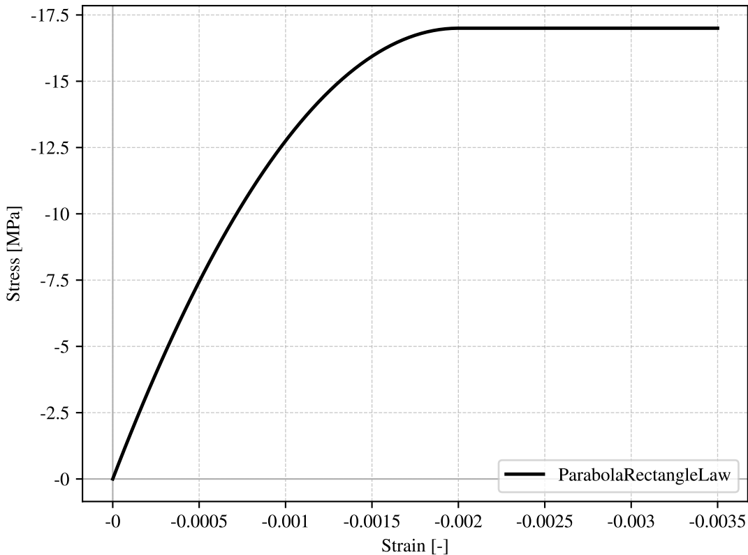
Constitutive Law of C30/37 ULS
