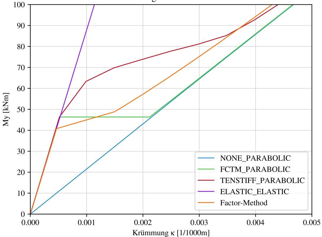
C.1_3 with different constitutive laws M-K-Diagram at x = 0.5 \cdot L
