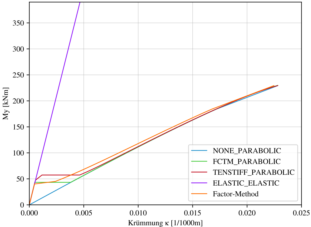
C.1_3 with different constitutive laws M-K-Diagram at x = 0.0 \cdot L
