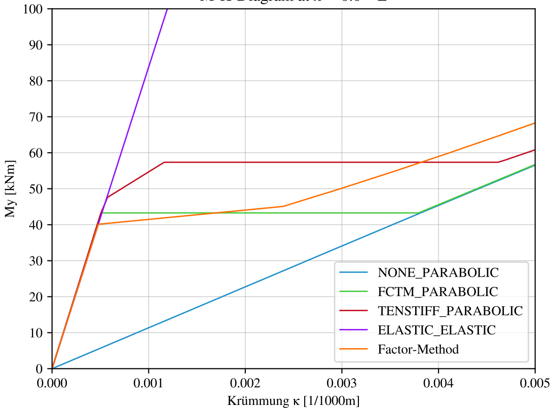
C.1_3 with different constitutive laws M-K-Diagram at x = 0.0 * L
