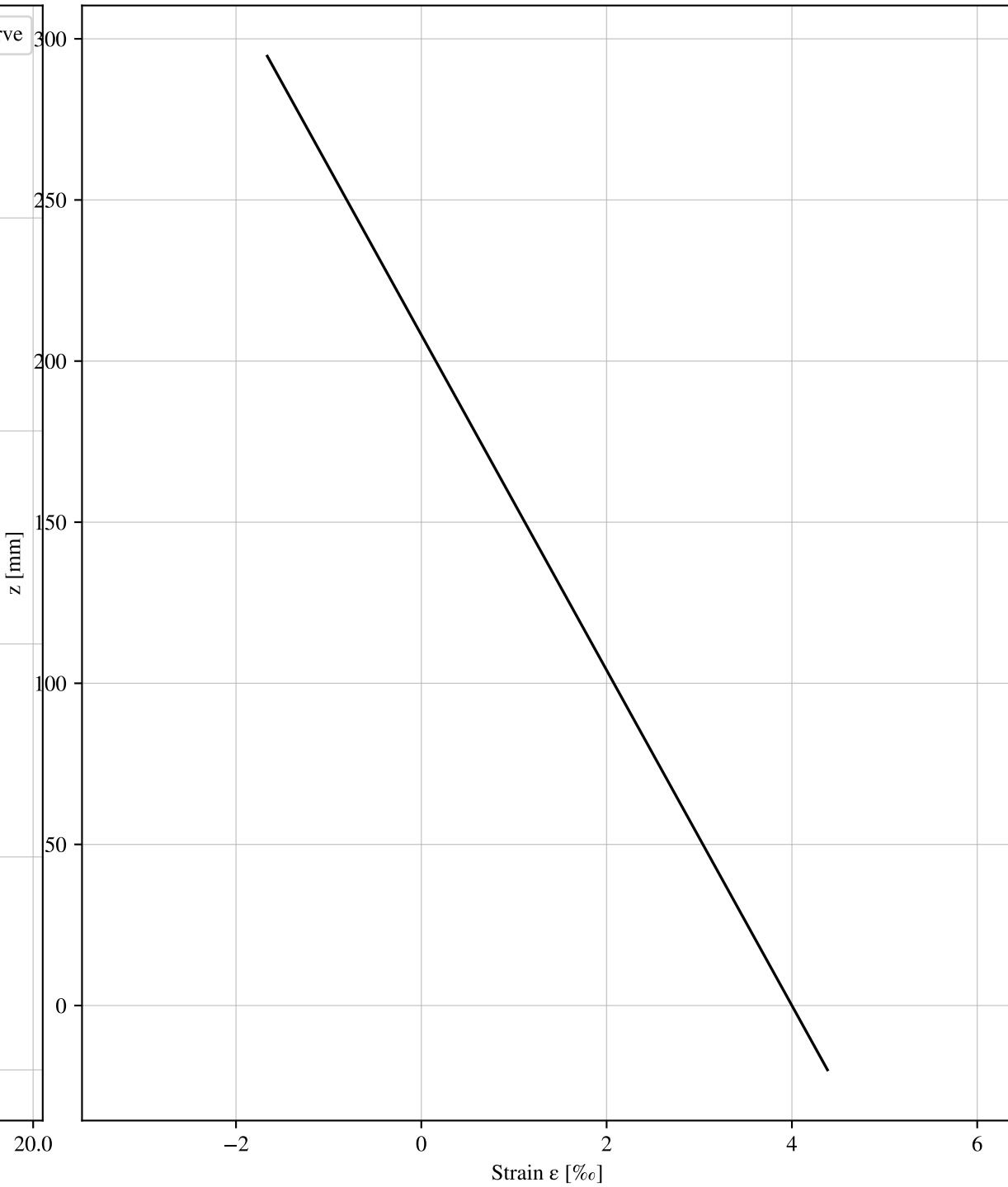
C.2 : Strain profile at breaking point of section at x = 0.5
