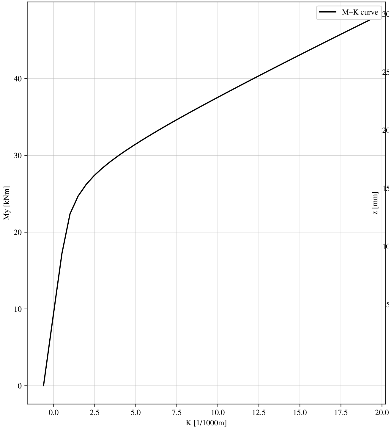
C.2: Moment-curvature-diagram for reinforcement governing section
