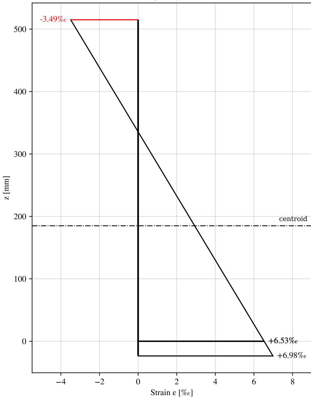
C.1_3: Strain profile at breaking point of section at x = 0.5 num_post_yield = 0
