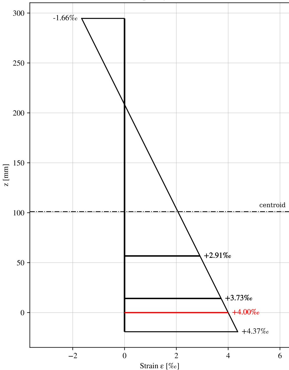
C.2 : Strain profile at breaking point of section at x = 0.5 num_post_yield = 0
