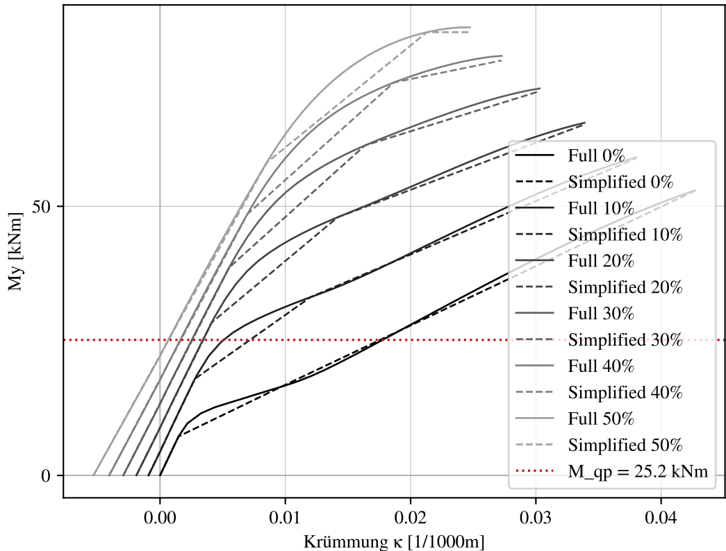
M-K-Diagrams at x_{\text{norm}} = 0.12 of C1_1 — full vs. simplified, varying prestress
