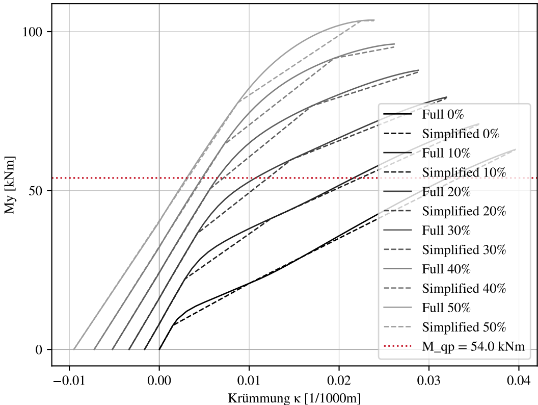
M-K-Diagrams at x_{\text{norm}} = 0.38 of C1_1 — full vs. simplified, varying prestress
