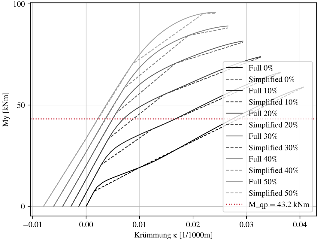
M-K-Diagrams at x_{\text{norm}} = 0.25 of C1_1 — full vs. simplified, varying prestress
