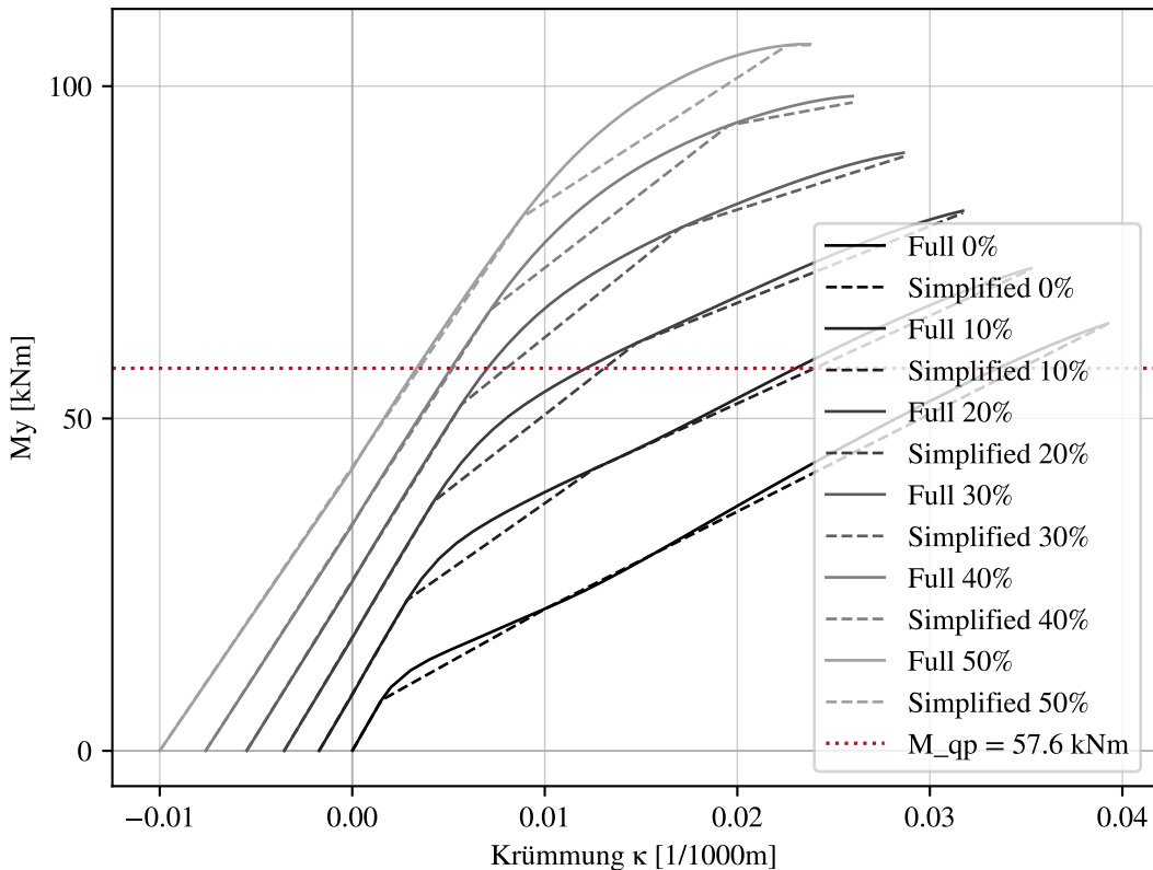
M-K-Diagrams at midspan of C1_1 — full vs. simplified, varying prestress
