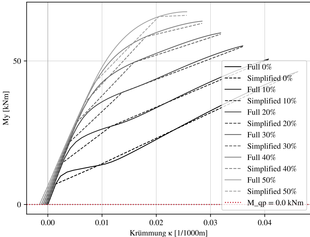
M-K-Diagrams at support of C1_1 — full vs. simplified, varying prestress
