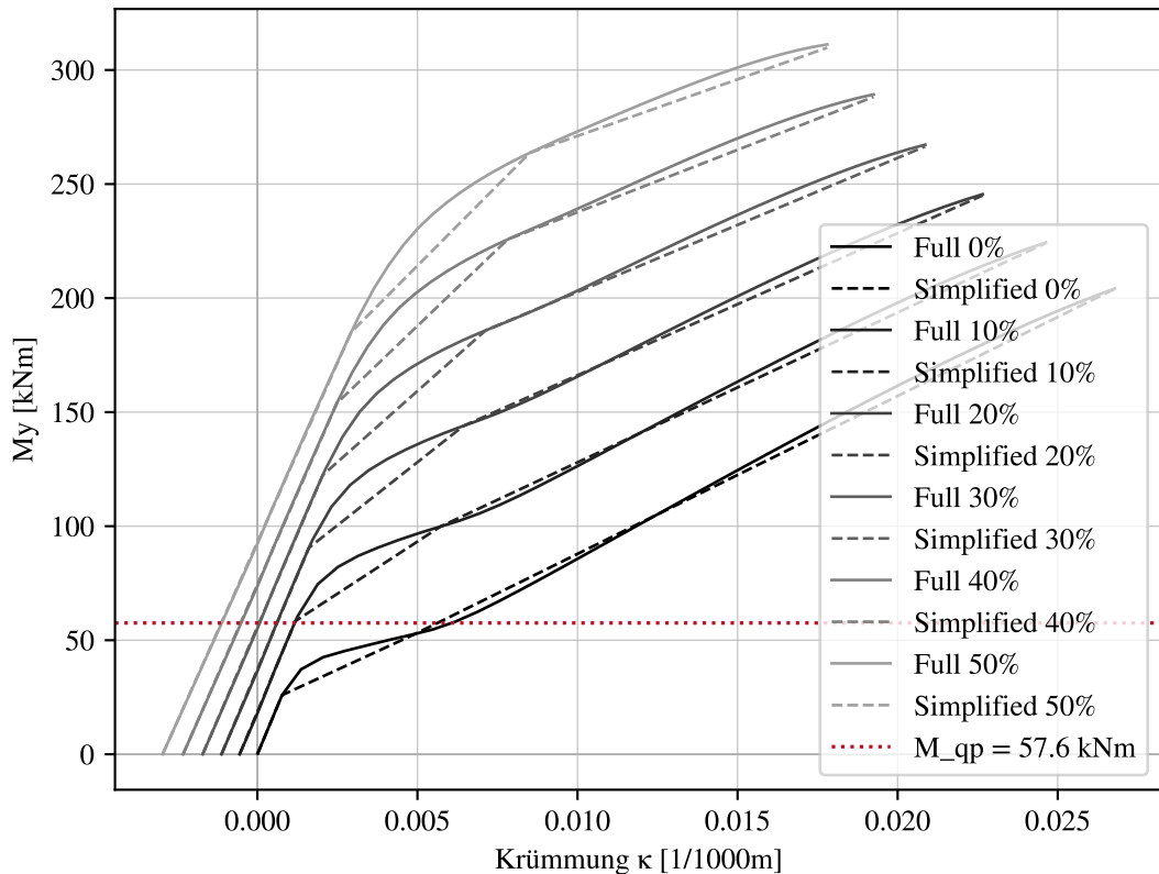
M-K-Diagrams at midspan of C1_2_1 — full vs. simplified, varying prestress
